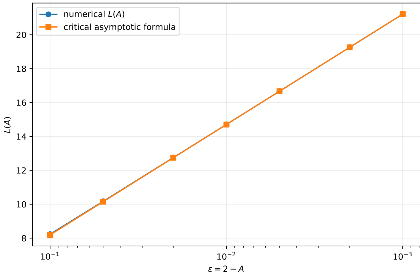
Logarithmic width divergence as A \rightarrow 2^-
