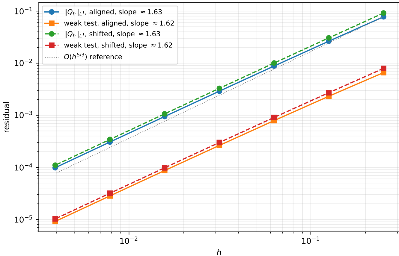
Mesh convergence of the residual, zero-energy cusp compacton
