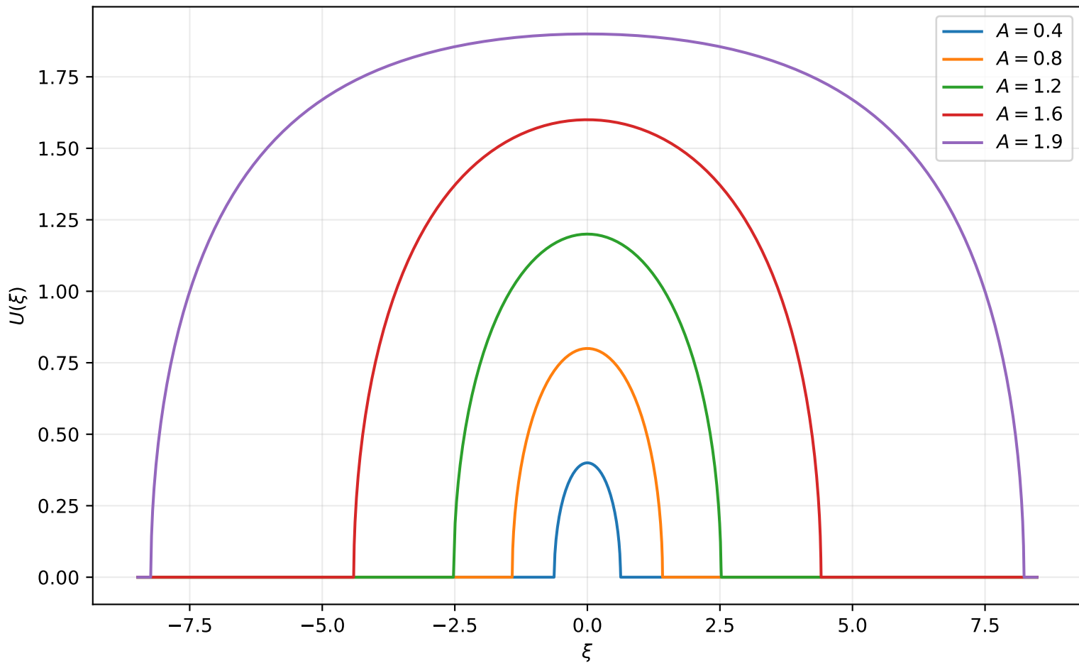
Nonzero-energy cusp compactons: m = 2, n = 1, a = 1, b = 2, 0 < A < 2
