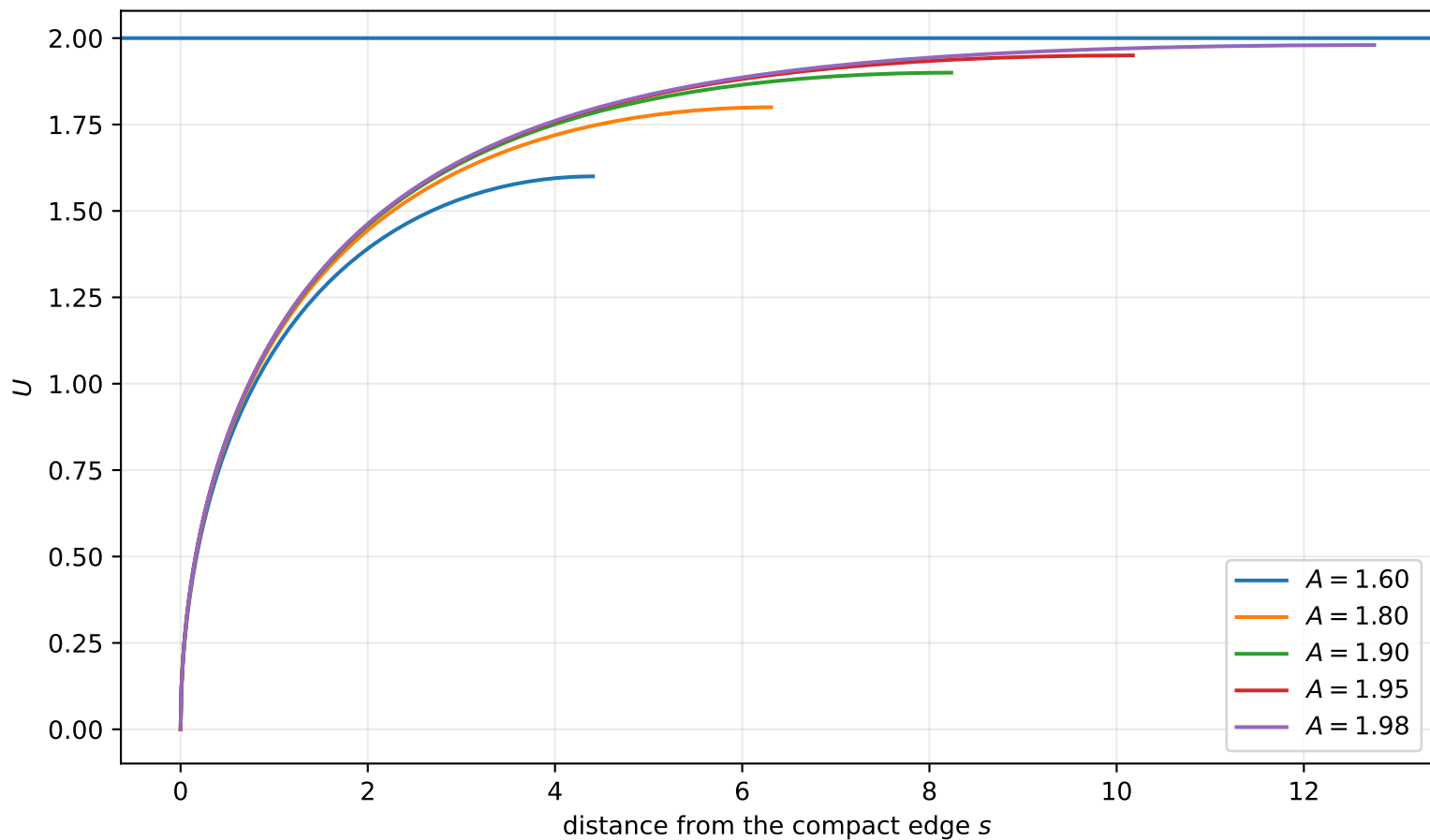
Critical broadening as A \rightarrow 2^-
