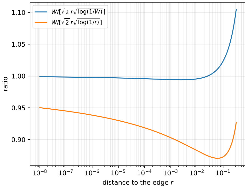
Logarithmically corrected edge law
