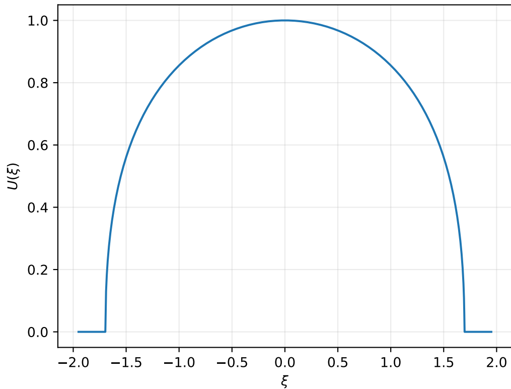
Critical compacton: m = 2, n = 1, a = 3, b = 2, E = -1
