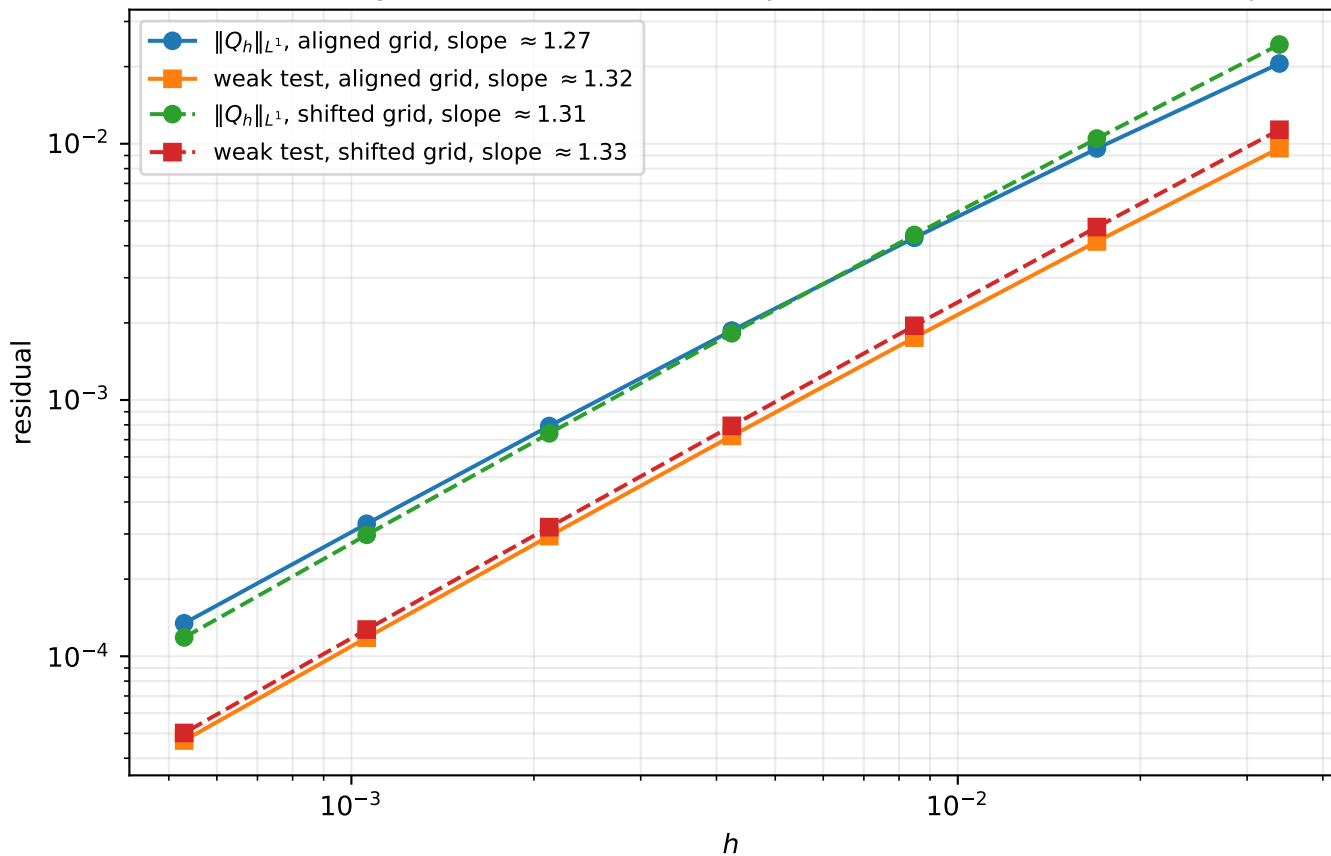
Mesh convergence of the extended-operator residual, critical example
