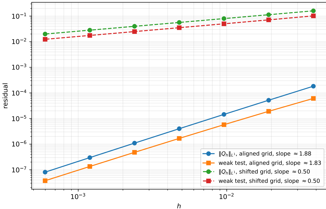
Mesh convergence of the weak residual, A = 1
