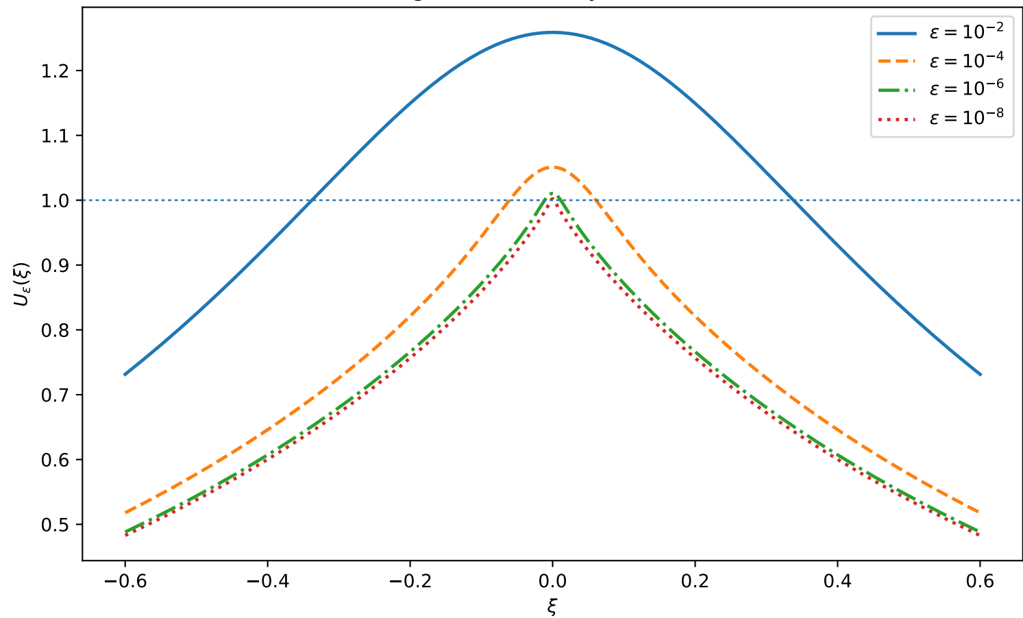
Regularized solitary-wave core
