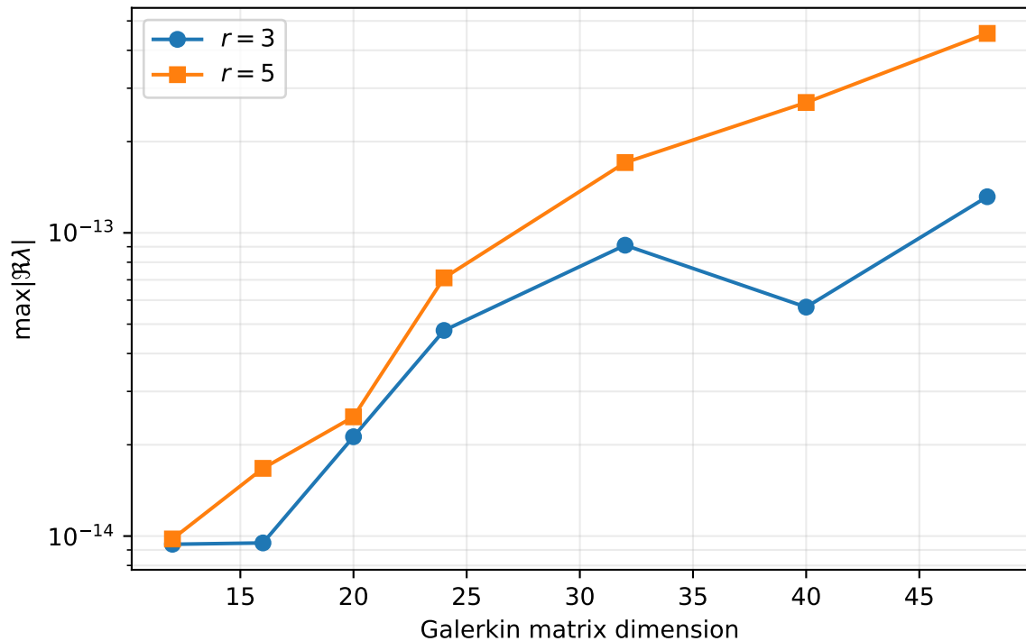
Jacobi-Galerkin generator: real parts at roundoff scale
