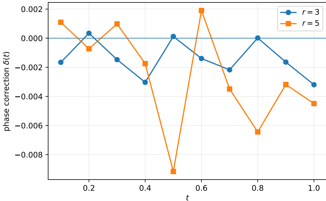
Phase error relative to speed c = 1 , N = 384
