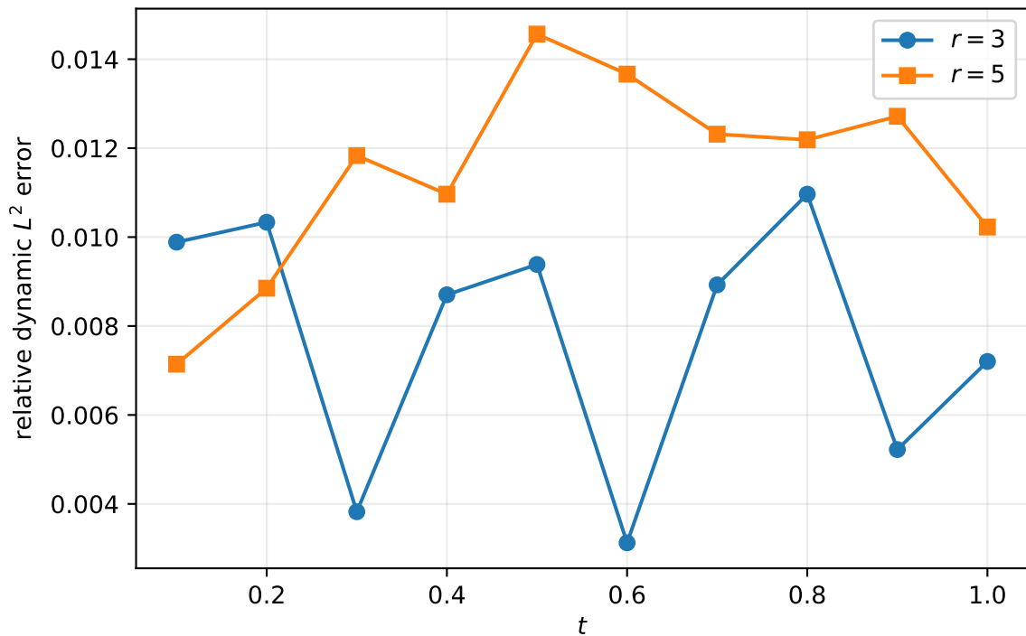
Projected-shape propagation error, p = 2 , c = \mu = 1 , N = 384
