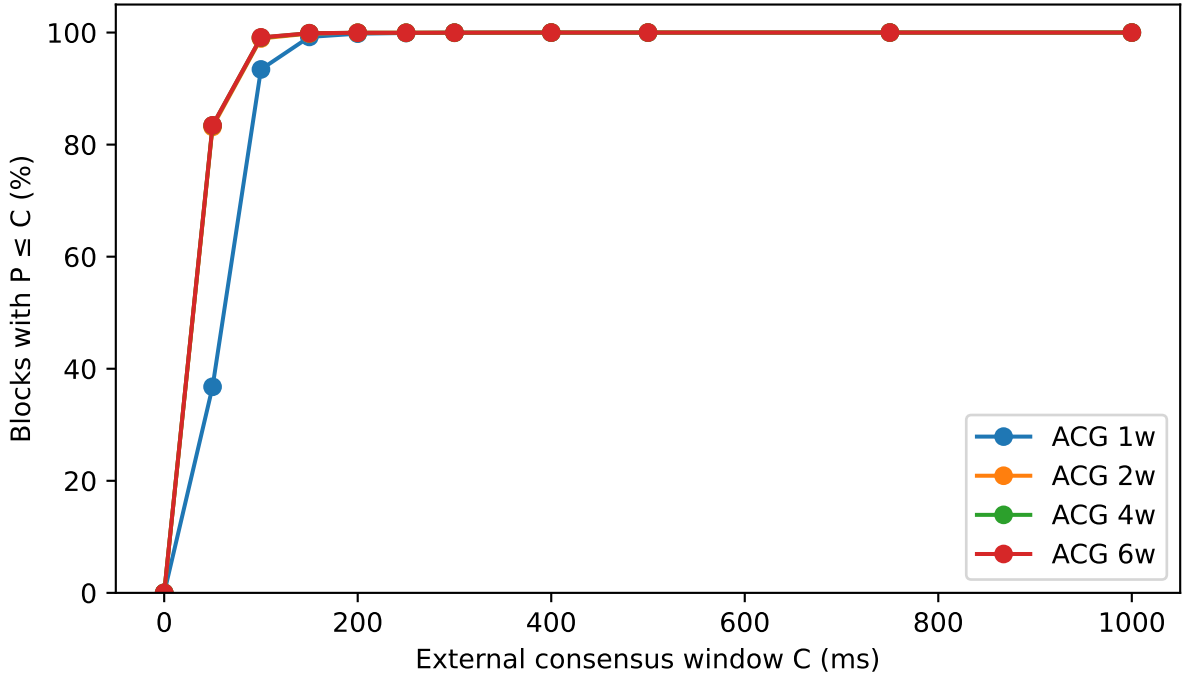
S1-derived Wasmd consensus-window sensitivity: pre-consensus completion coverage
