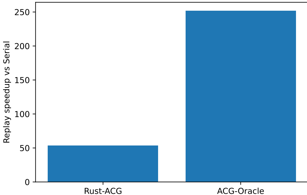
S3 current ACG vs perfect-access oracle (6 workers)
