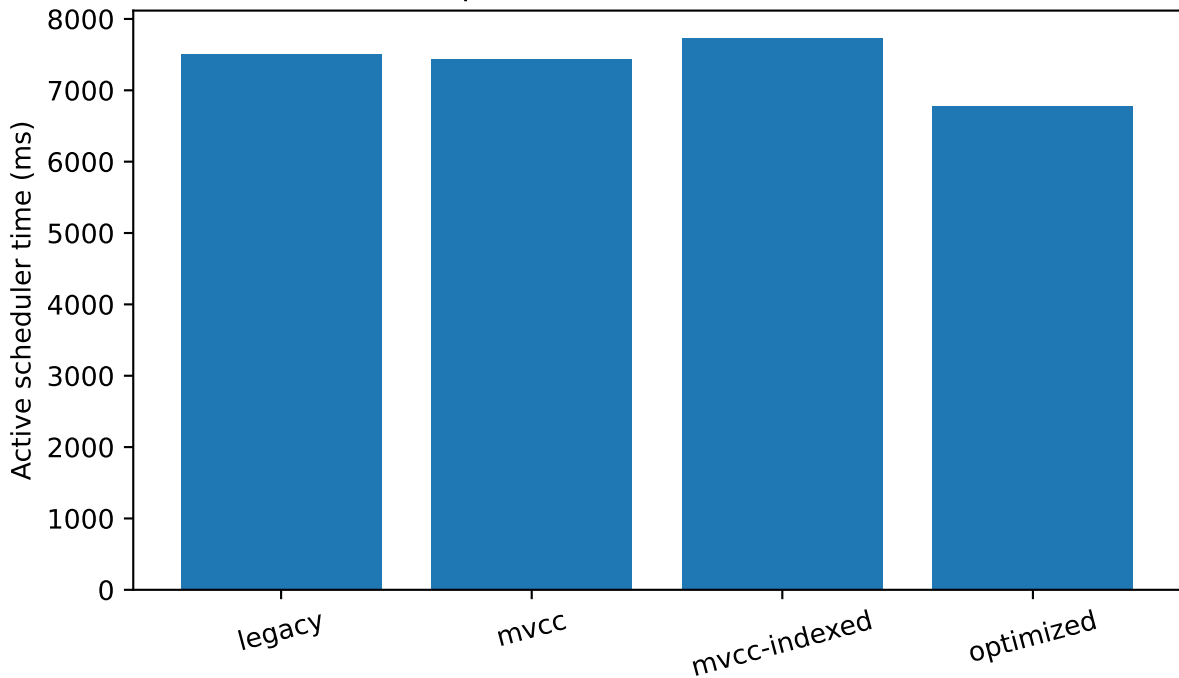
Rust-ACG implementation ablation, S3, 6 workers
