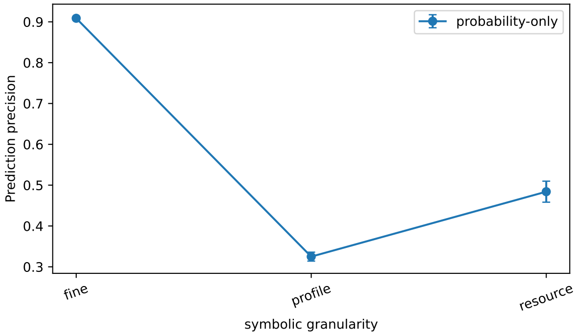
Symbolic granularity vs prediction precision
