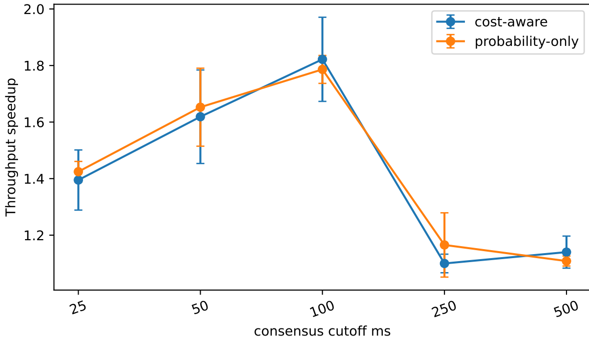
Consensus cutoff under candidate/decided divergence
