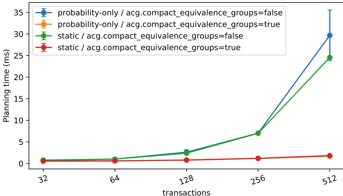
Planning cost with/without graph compaction
