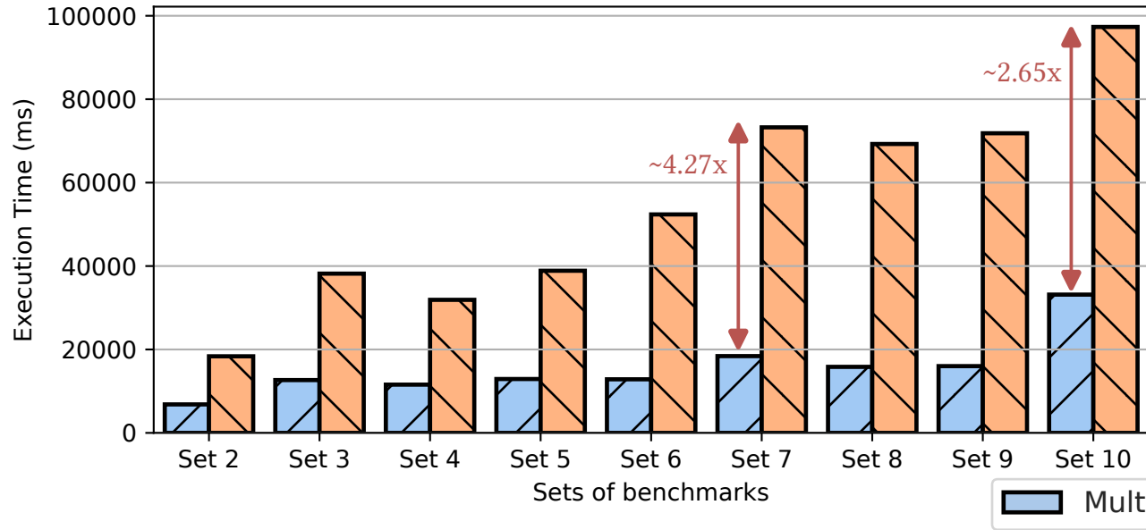
a) Execution time
