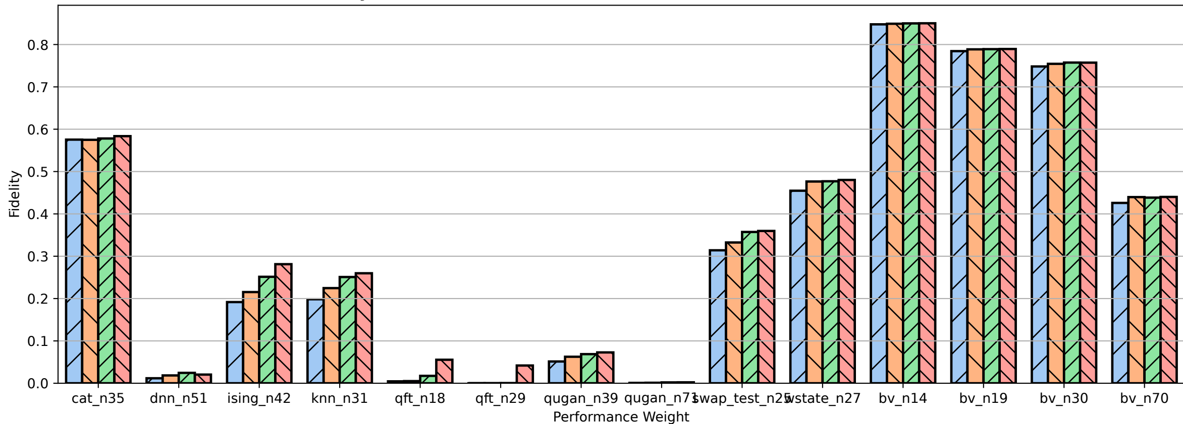
MultiQ Planner Evaluation Fidelity
