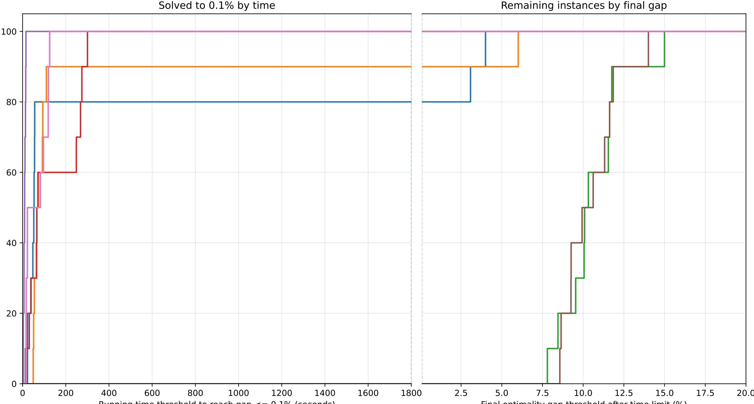
Joined runtime-gap performance profile — 20x20, Expected, alpha=0.03
