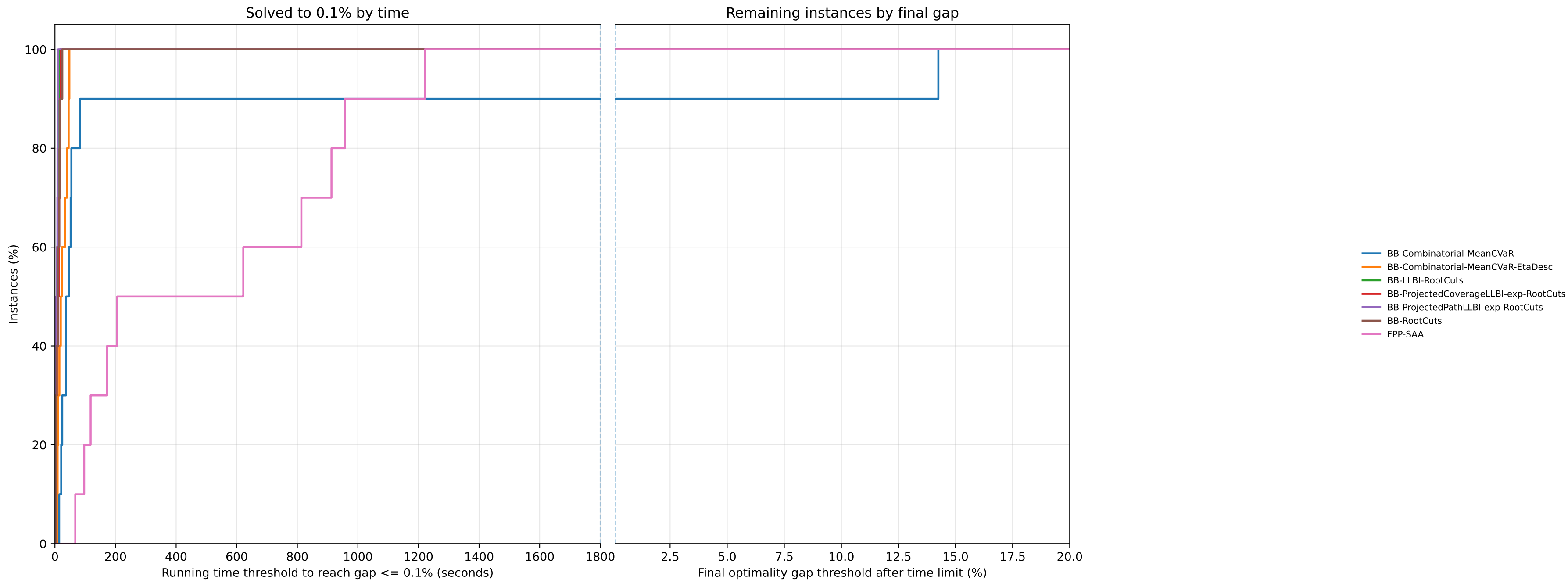
Joined runtime-gap performance profile — 20x20, MeanCVaR, alpha=0.01
