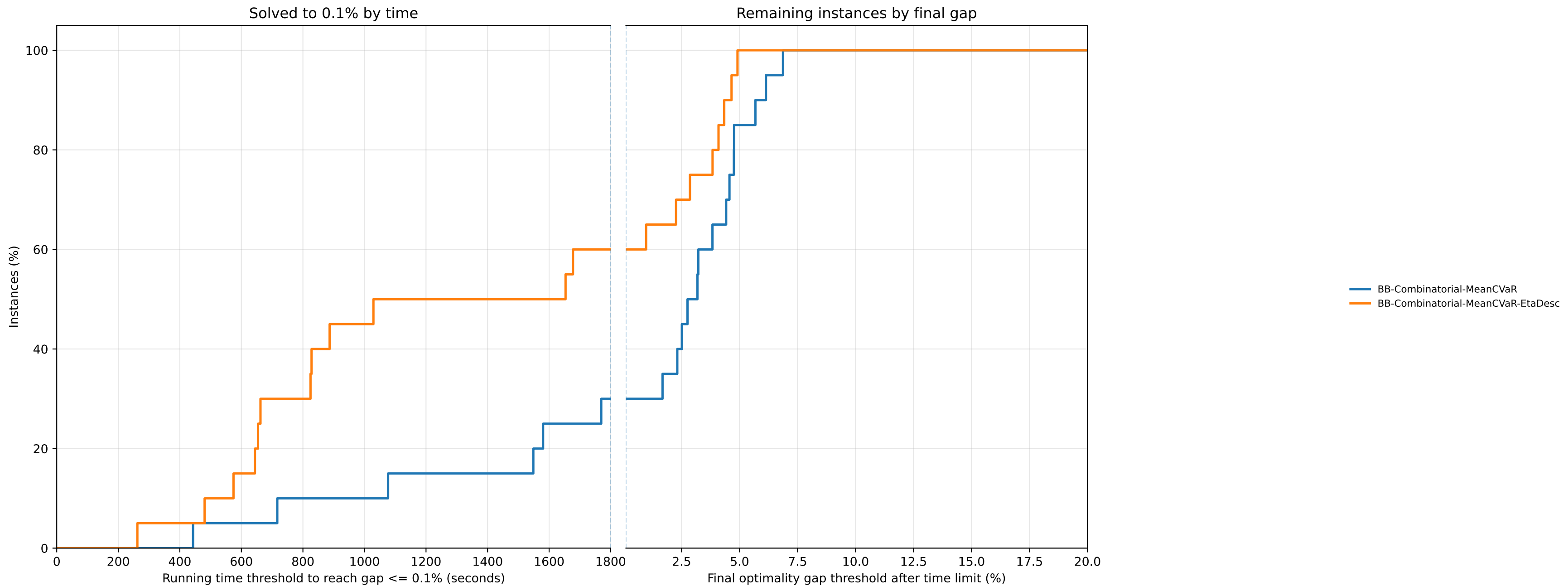
Joined runtime-gap performance profile — 20x20, MeanCVaR, selected methods 400/600, alpha=0.02
