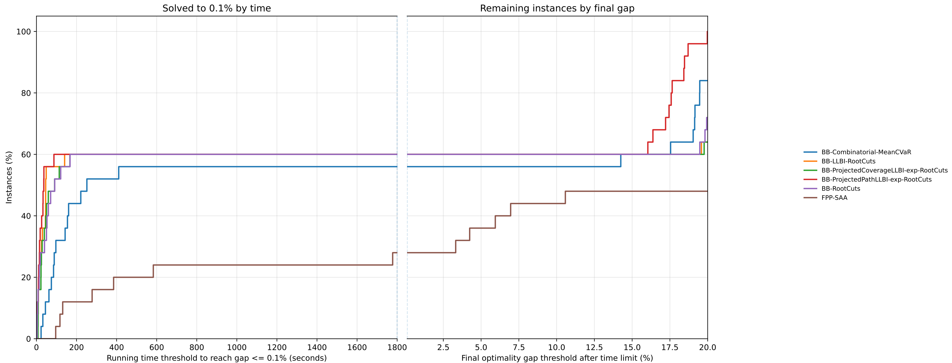
Joined runtime-gap performance profile — MeanCVaR, alpha=0.01 (1%)
