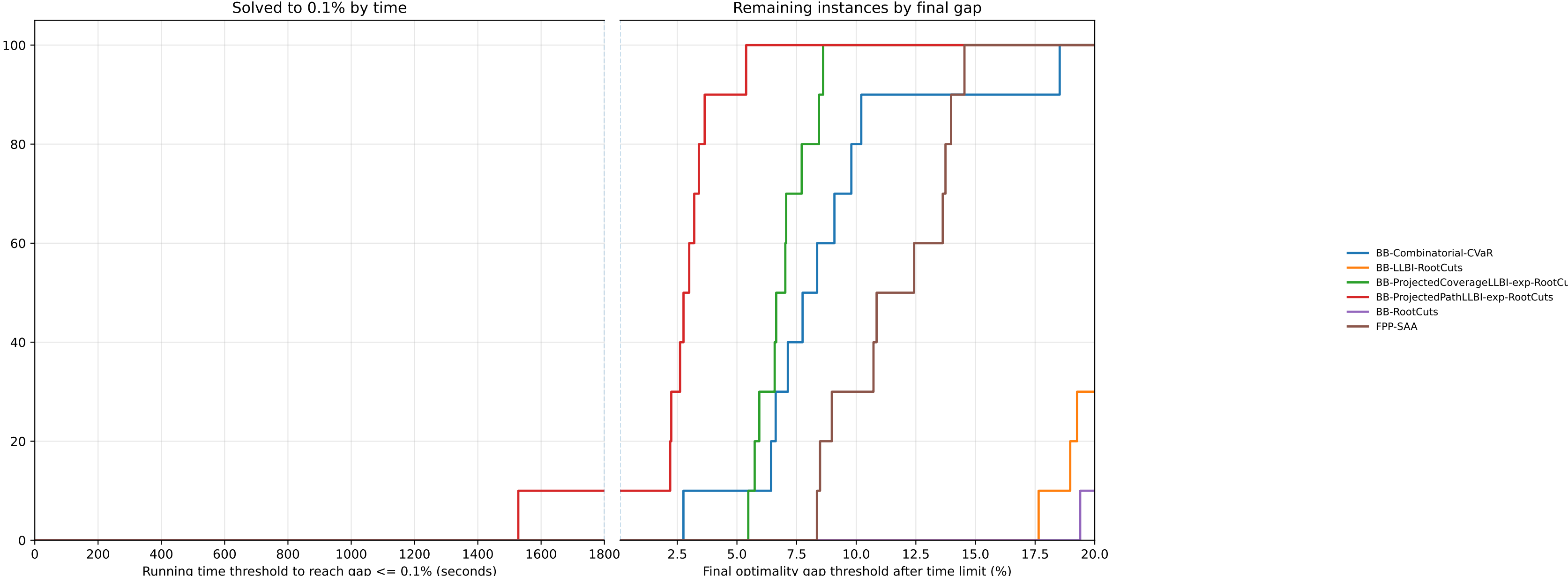
Joined runtime-gap performance profile — 20x20, cvar, alpha=0.03
