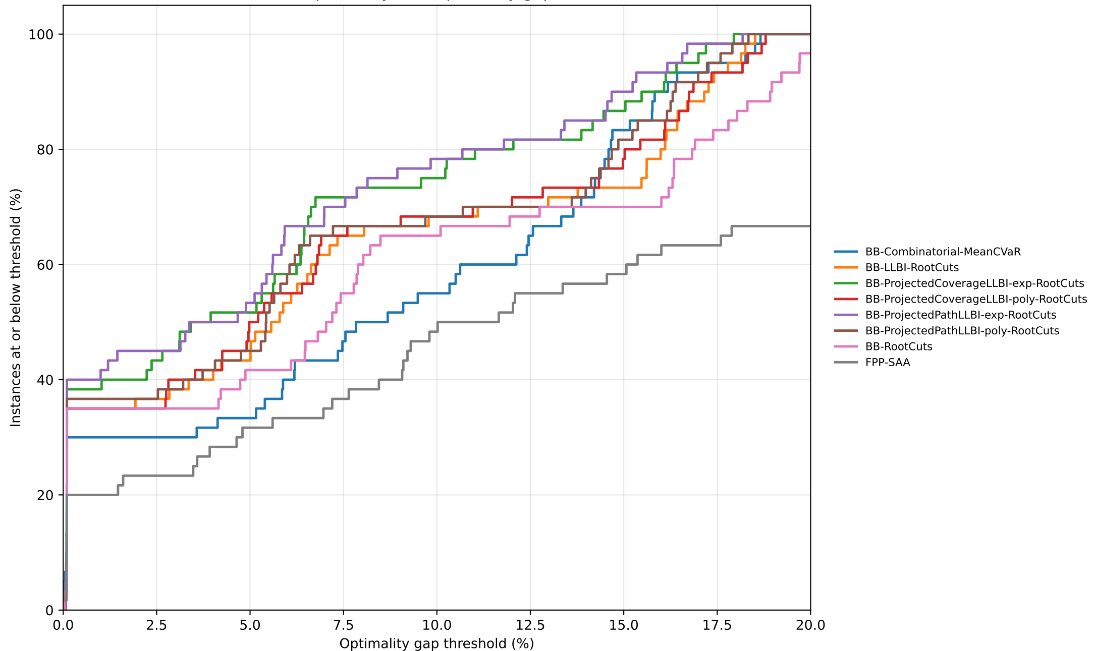
Performance profile by final optimality gap — MeanCVaR
