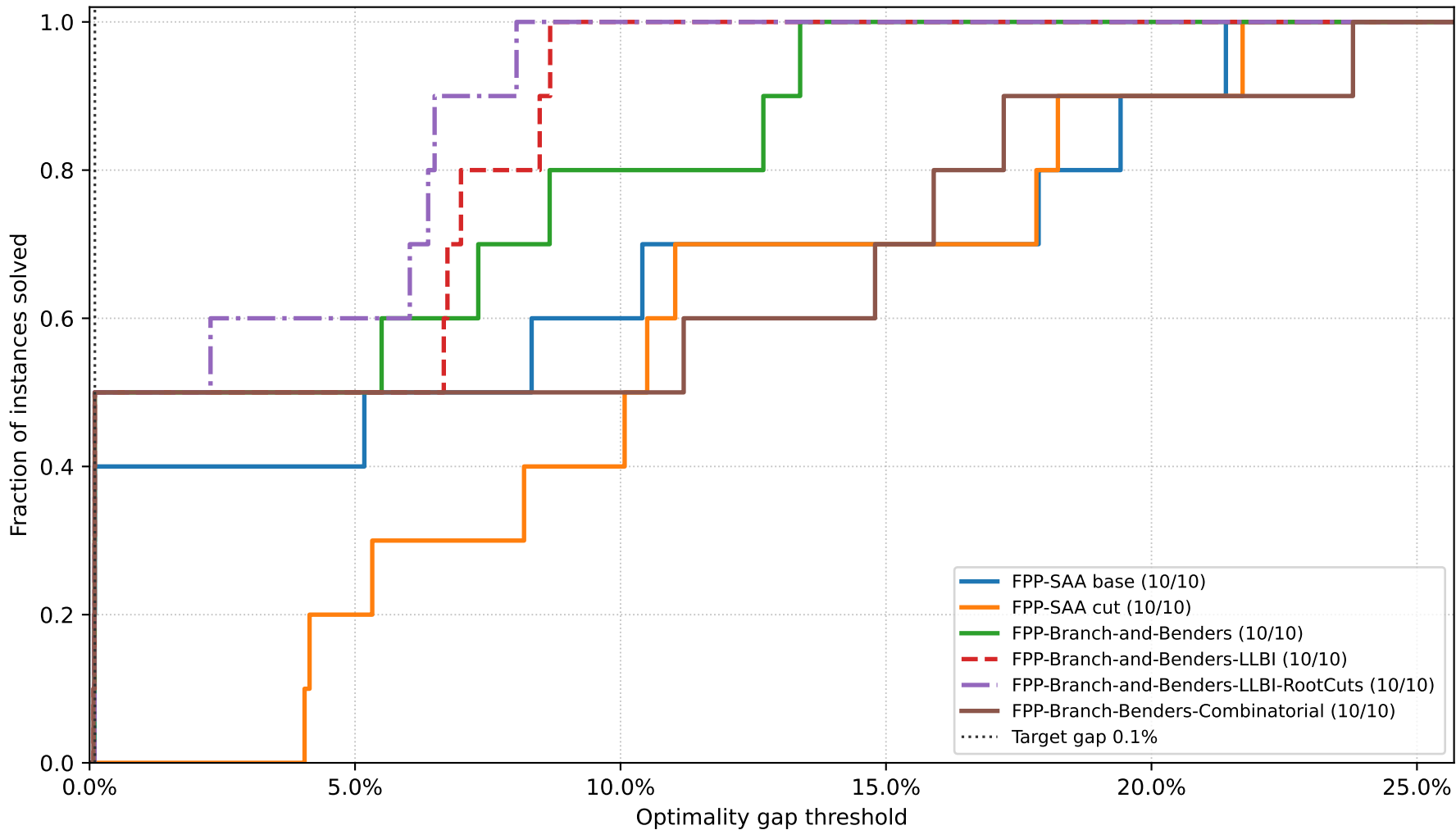
Sub20 Optimality-Gap Profile - CVaR Objective
