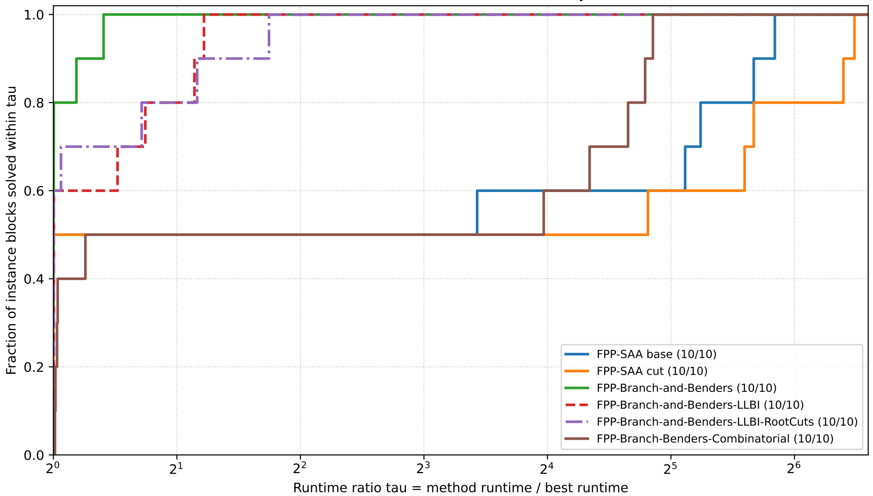
Sub20 Performance Profile - CVaR Objective
