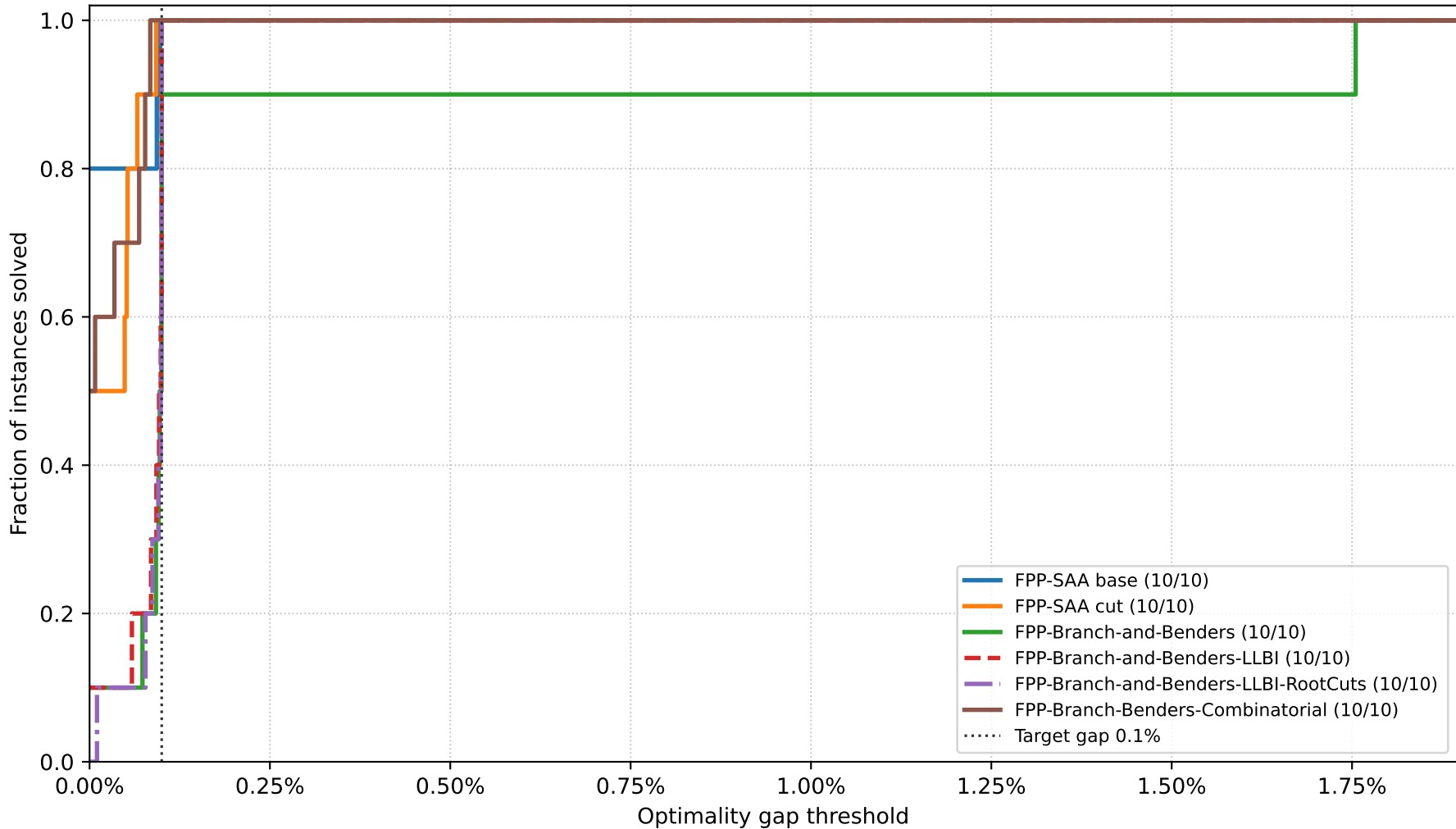
Sub20 Optimality-Gap Profile - Expected Objective
