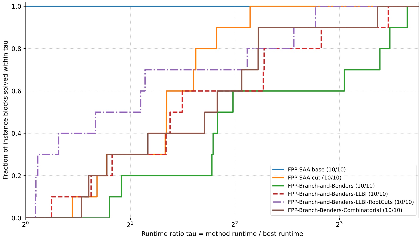
Sub20 Performance Profile - Expected Objective
