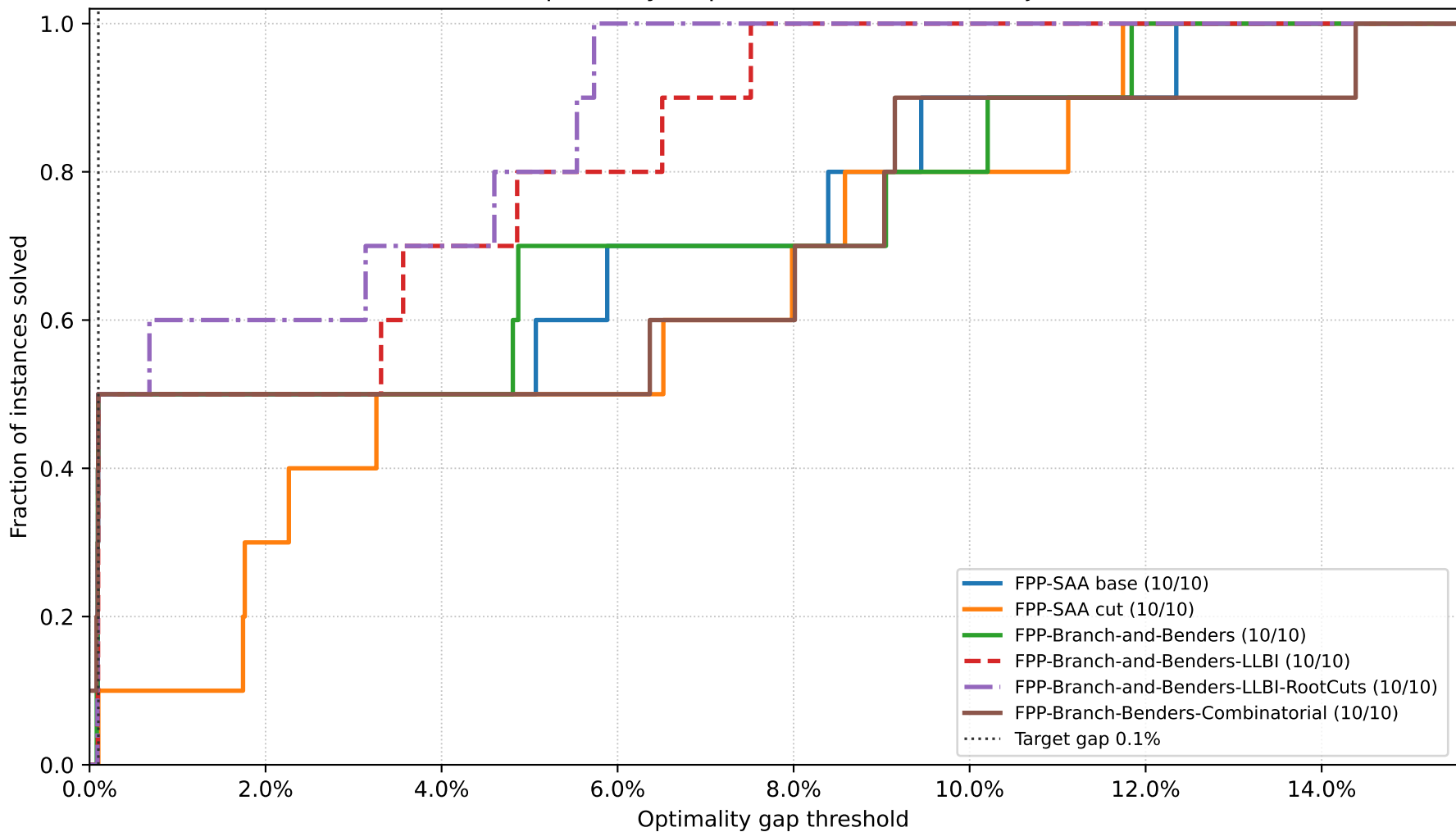
Sub20 Optimality-Gap Profile - MeanCVaR Objective
