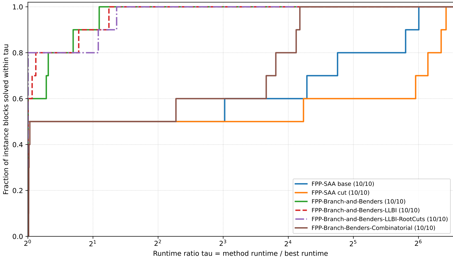
Sub20 Performance Profile - MeanCVaR Objective
