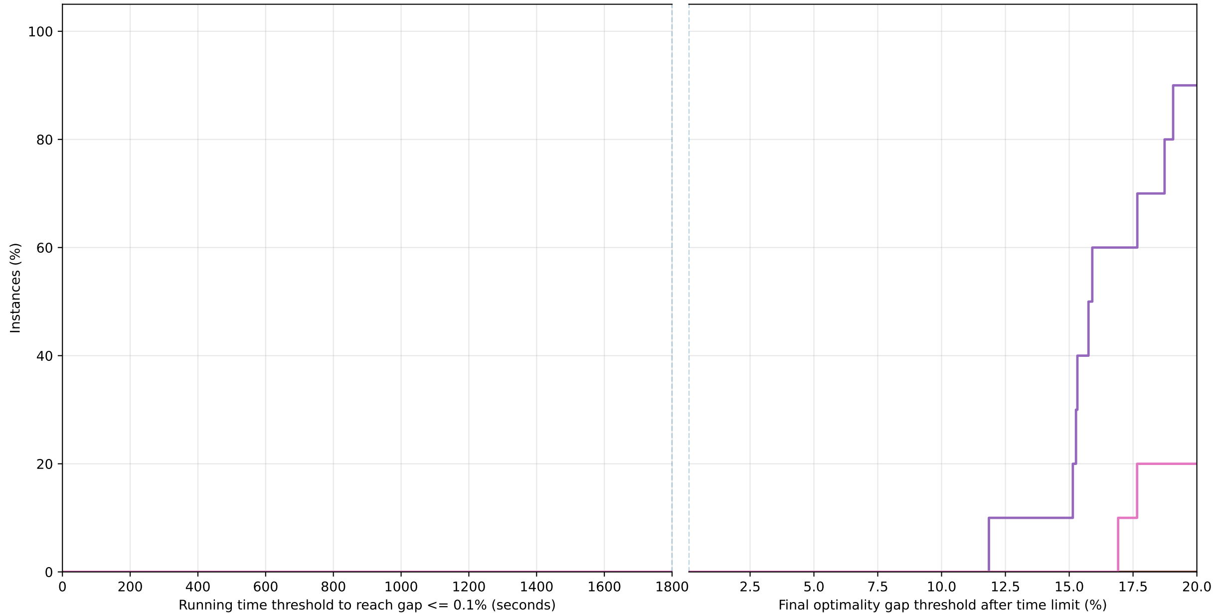
Solved to 0.1% by time
