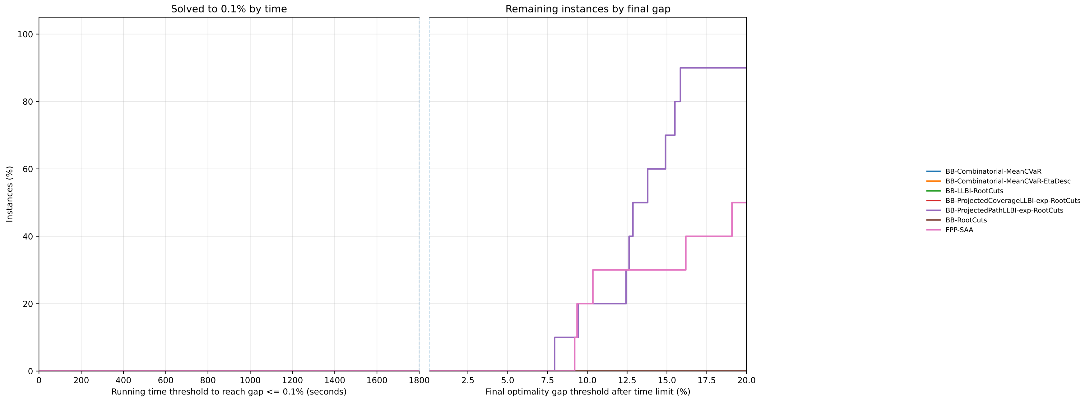
Joined runtime-gap performance profile — 40x40, MeanCVaR, alpha=0.03
