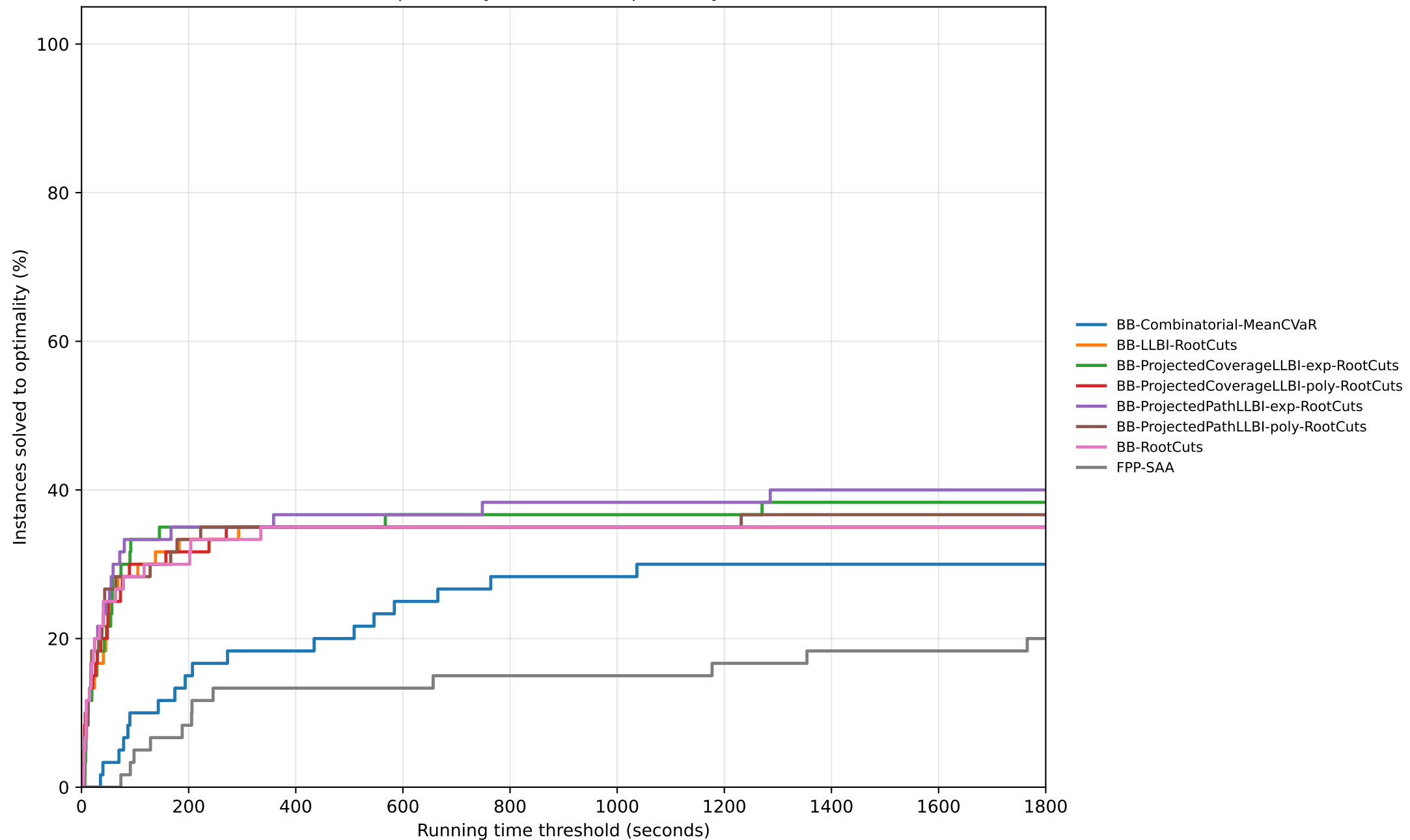
Performance profile by runtime to optimality — MeanCVaR
