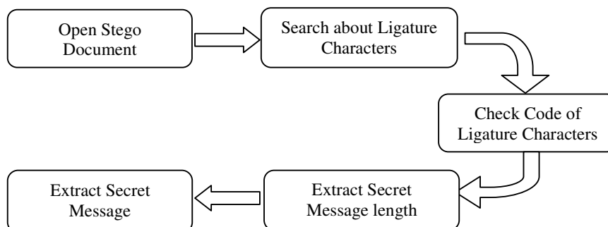
Figure 3: Extracting Process
