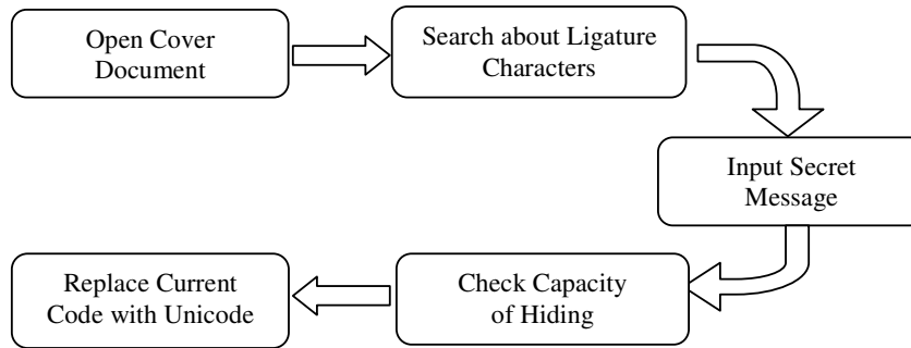
Figure 2: Hiding Process
