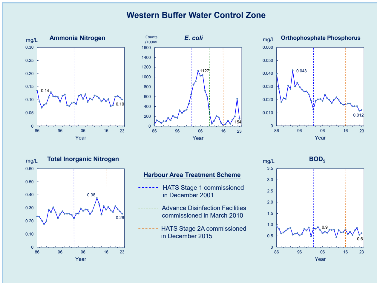
Figure 19. Long-term water quality trends in the Western Buffer WCZ, 1986-2023
