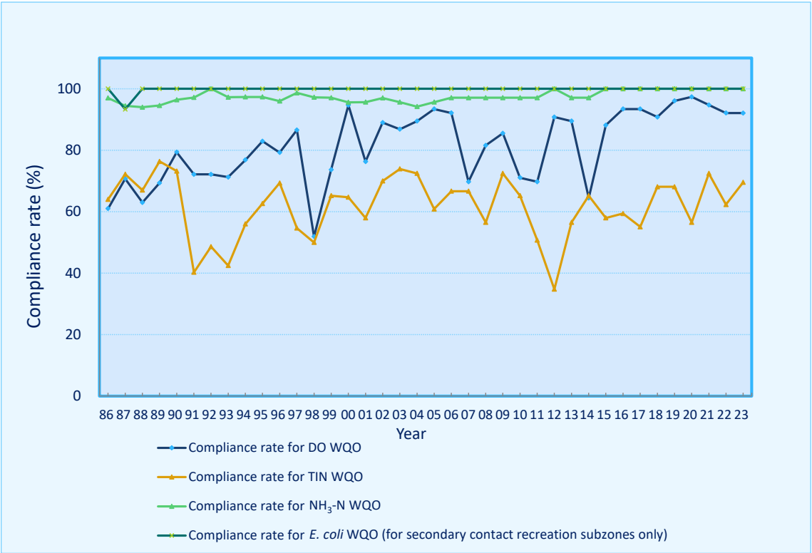
Figure 2. Compliance rates for four key marine WQOs, 1986-2023
