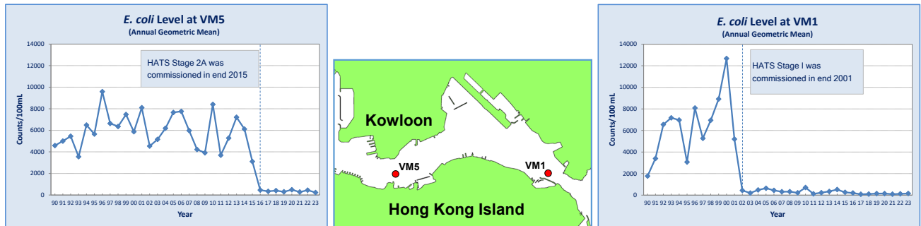
Figure 11. E. coli level at the central (VM5) and eastern (VM1) parts of the Victoria Harbour WCZ, 1990-2023
