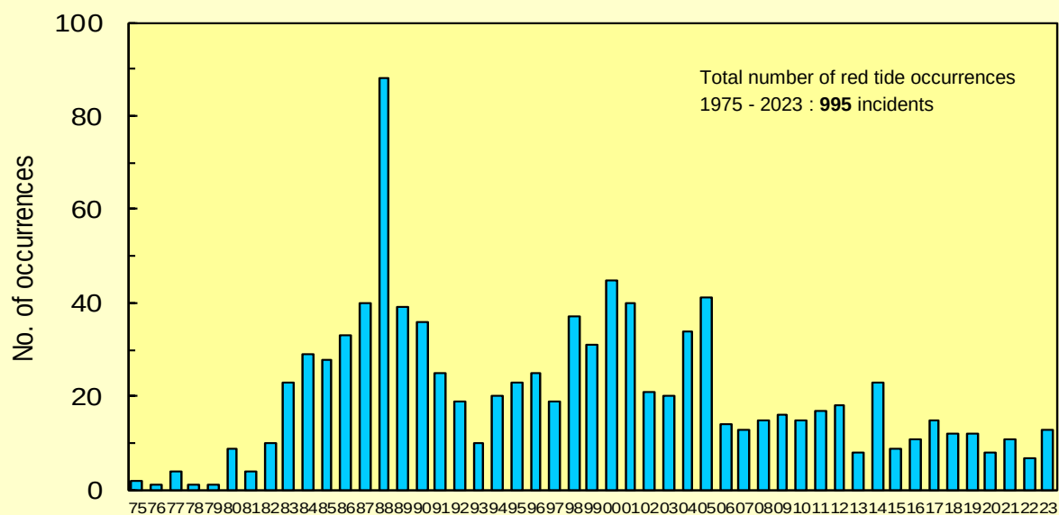
Yearly Distribution
