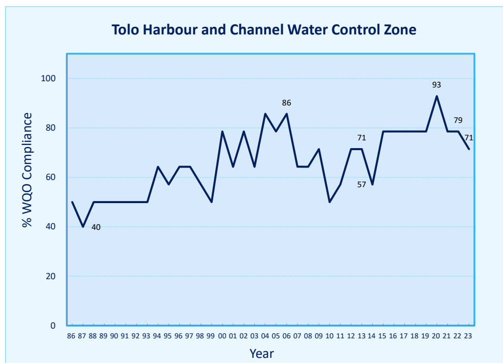
Figure 9. Overall WQO compliance rate for the Tolo Harbour and Channel WCZ, 1986-2023
