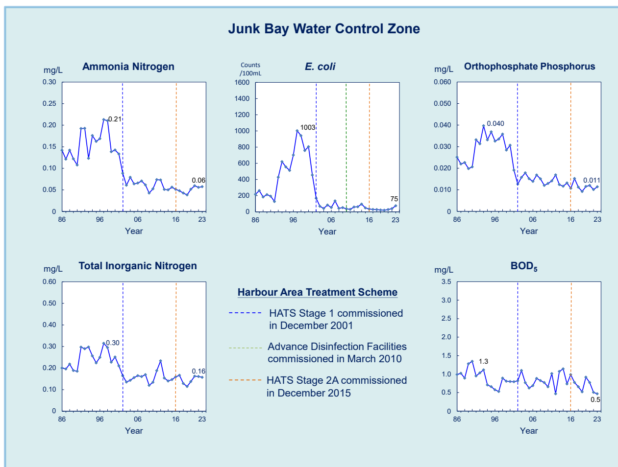
Figure 17. Long-term water quality trends in the Junk Bay WCZ, 1986-2023
