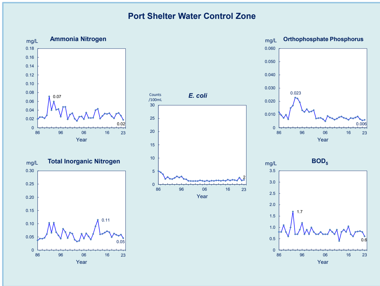
Figure 8. Long-term water quality trends in the Port Shelter WCZ, 1986-2023
