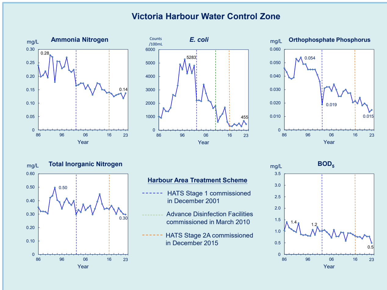
Figure 13. Long-term water quality trends in the Victoria Harbour WCZ, 1986-2023
