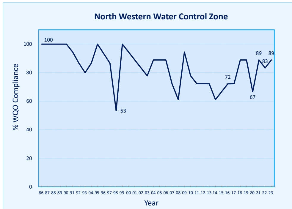
Figure 23. Overall WQO compliance for the North Western WCZ, 1986-2023
