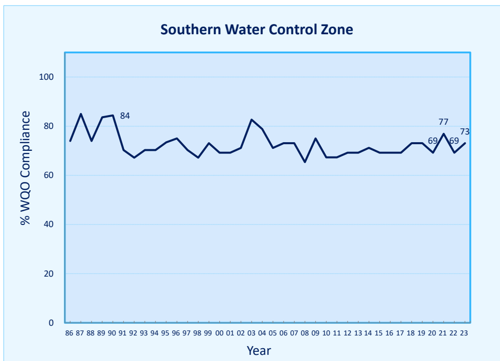
Figure 25. Overall WQO compliance for the Southern WCZ, 1986-2023
