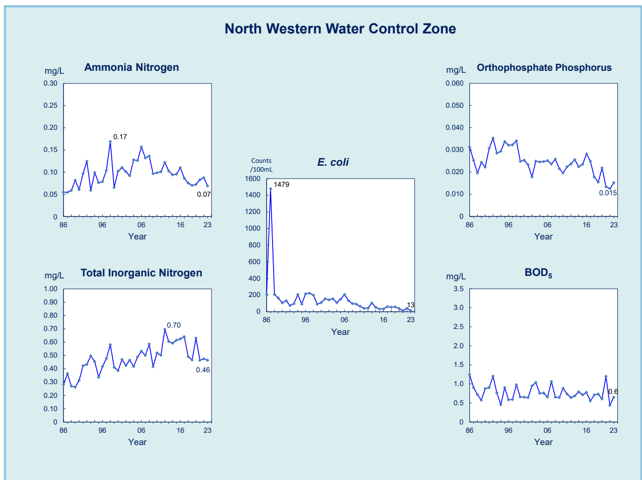
Figure 24. Long-term water quality trends in the North Western WCZ, 1986-2023
