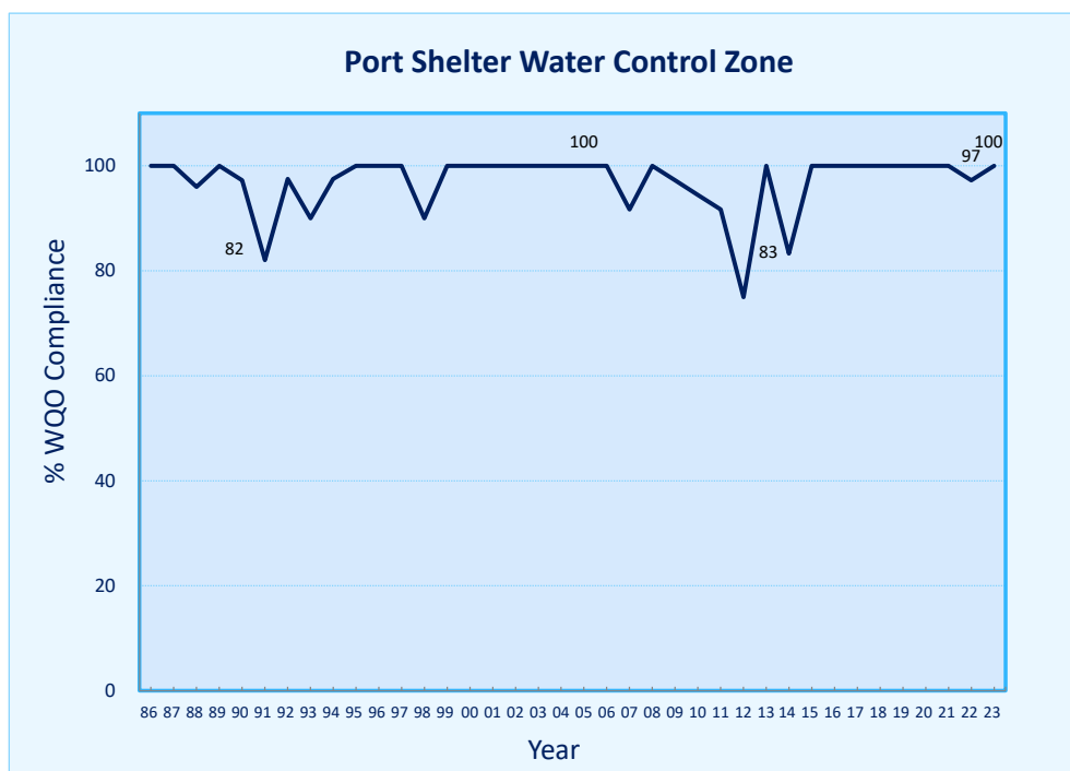
Figure 7. Overall WQO compliance rate for the Port Shelter WCZ, 1986-2023
