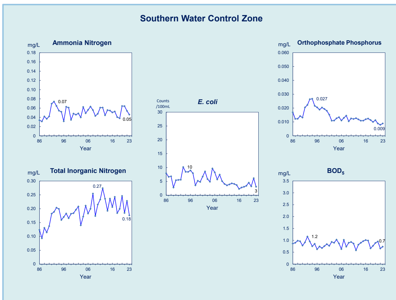
Figure 26. Long-term water quality trends in the Southern WCZ, 1986-2023
