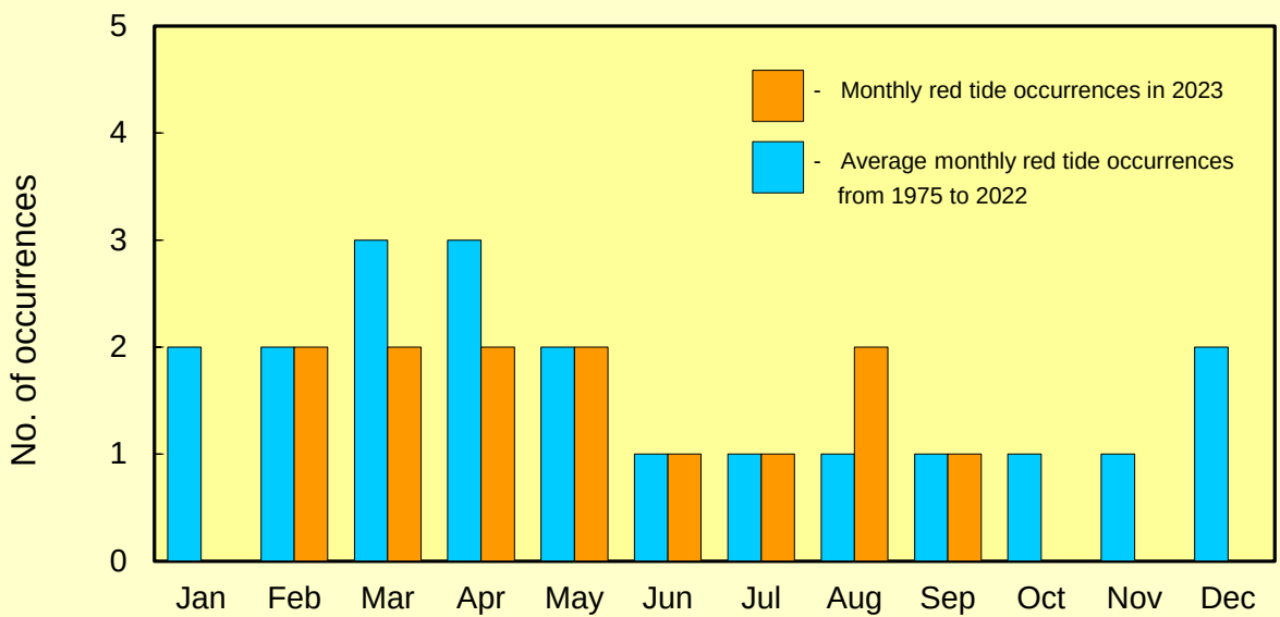
Monthly Distribution
