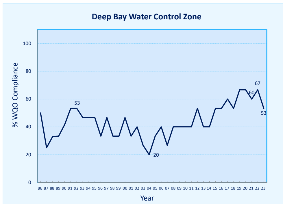
Figure 20. Overall WQO compliance for the Deep Bay WCZ, 1986-2023
