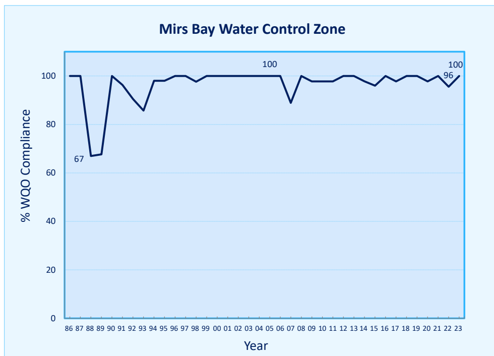
Figure 5. Overall WQO compliance rate for the Mirs Bay WCZ, 1986-2023
