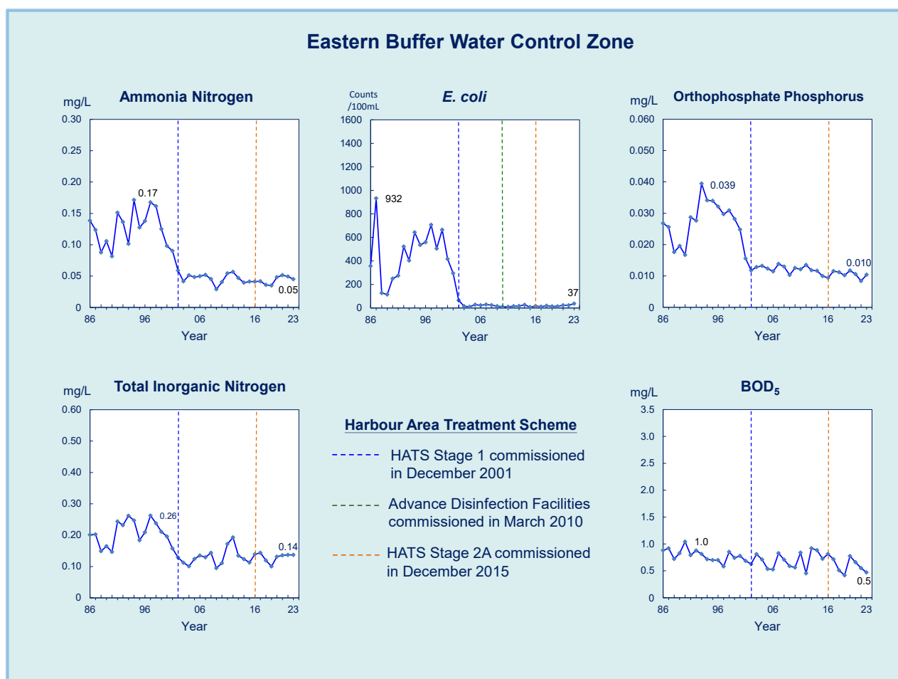
Figure 15. Long-term water quality trends in the Eastern Buffer WCZ, 1986-2023
