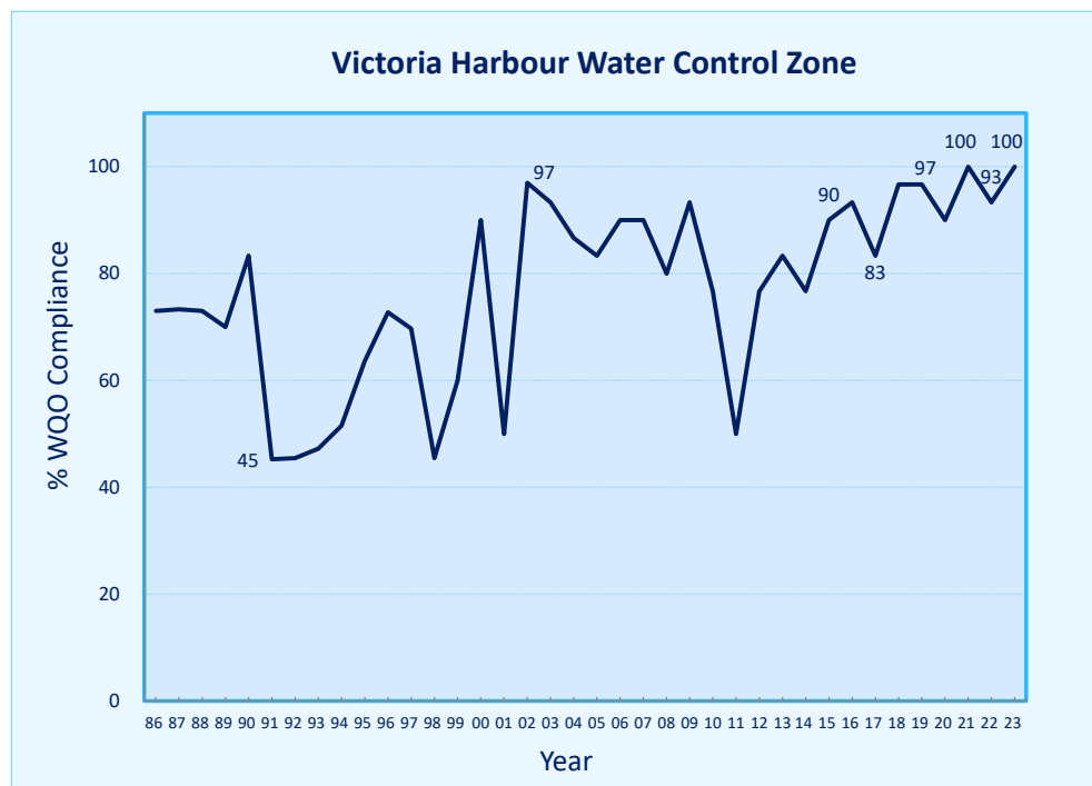
Figure 12. Overall WQO compliance rate for the Victoria Harbour WCZ, 1986-2023
