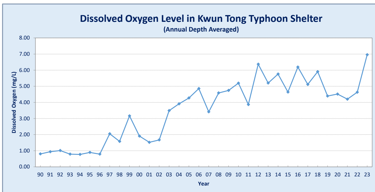
Figure 27. Long-term improvement in dissolved oxygen level in Kwun Tong Typhoon Shelter, 1990-2023
