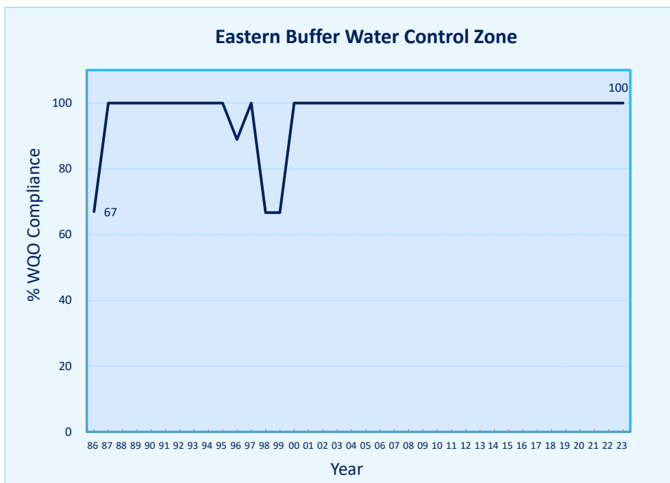
Figure 14. Overall WQO compliance rate for the Eastern Buffer WCZ, 1986-2023
