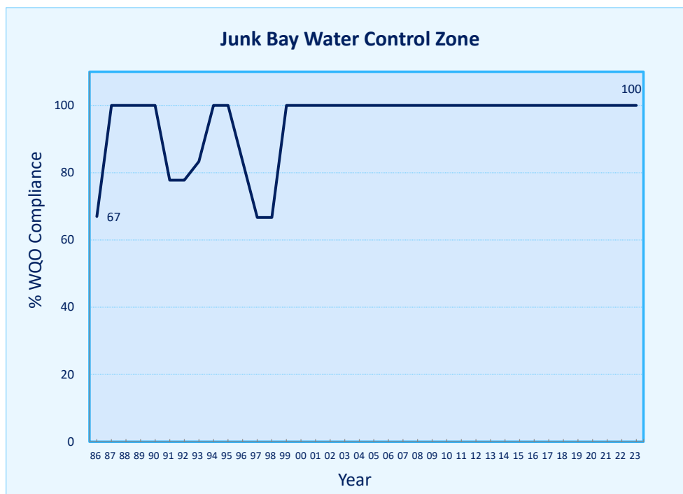
Figure 16. Overall WQO compliance rate for the Junk Bay WCZ, 1986-2023
