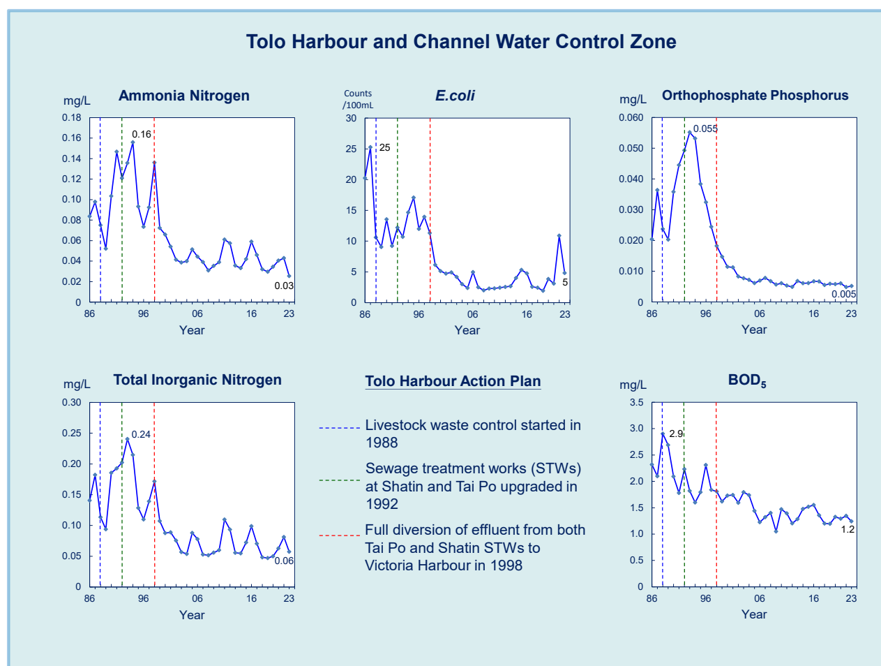
Figure 10. Long-term water quality trends in the Tolo Harbour and Channel WCZ, 1986-2023
