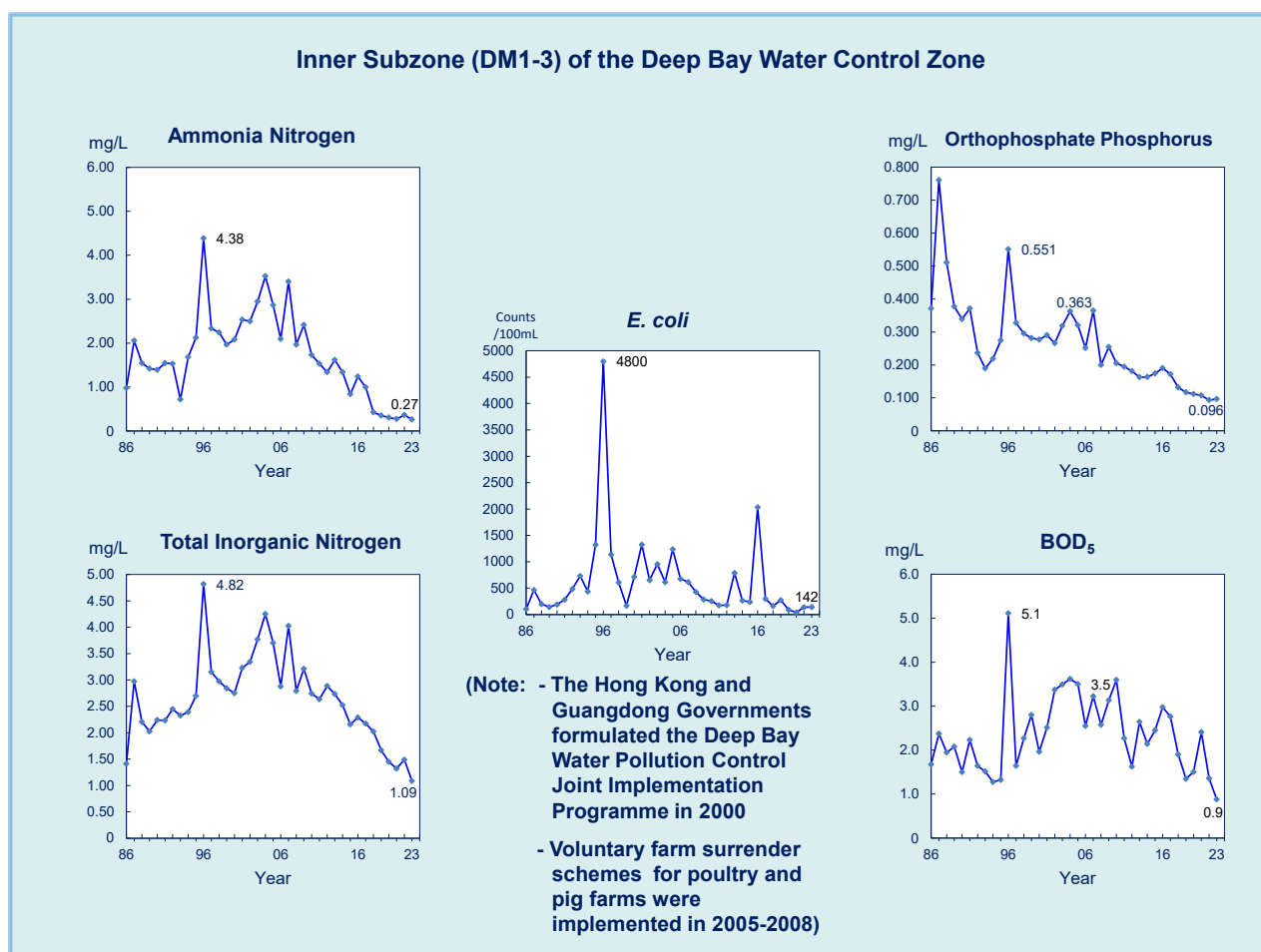
Figure 21. Long-term water quality trends in Inner Subzone of the Deep Bay WCZ, 1986-2023
