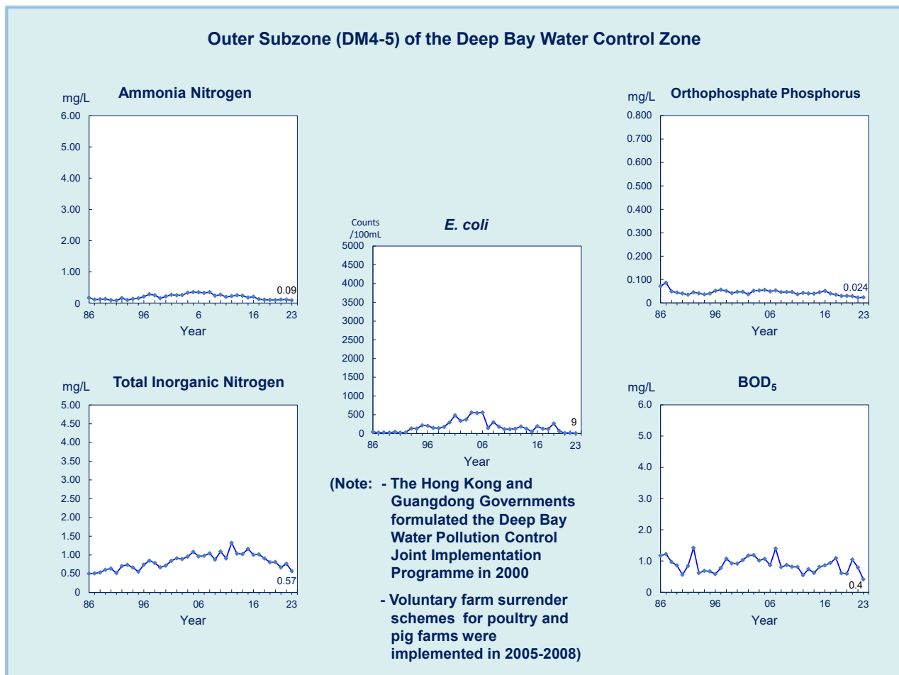
Figure 22. Long-term water quality trends Outer Subzone of the Deep Bay WCZ, 1986-2023
