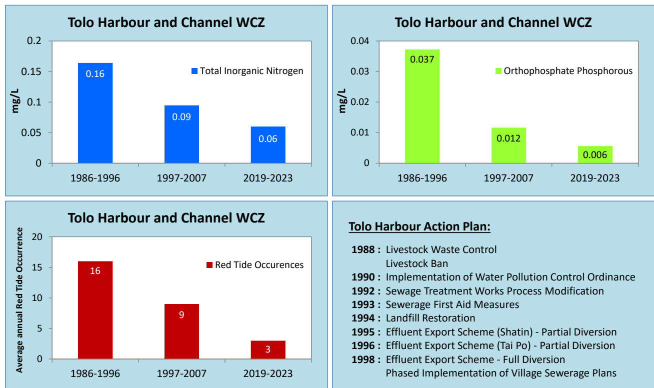
Figure 28. Reduction of nutrients levels with the average annual red tide occurrences in Tolo Harbour, 1986-2023
