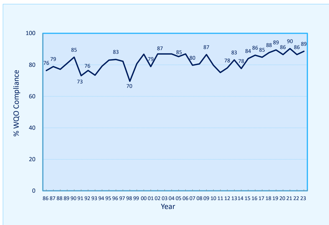
Figure 1. Overall marine WQO compliance rates, 1986-2023
