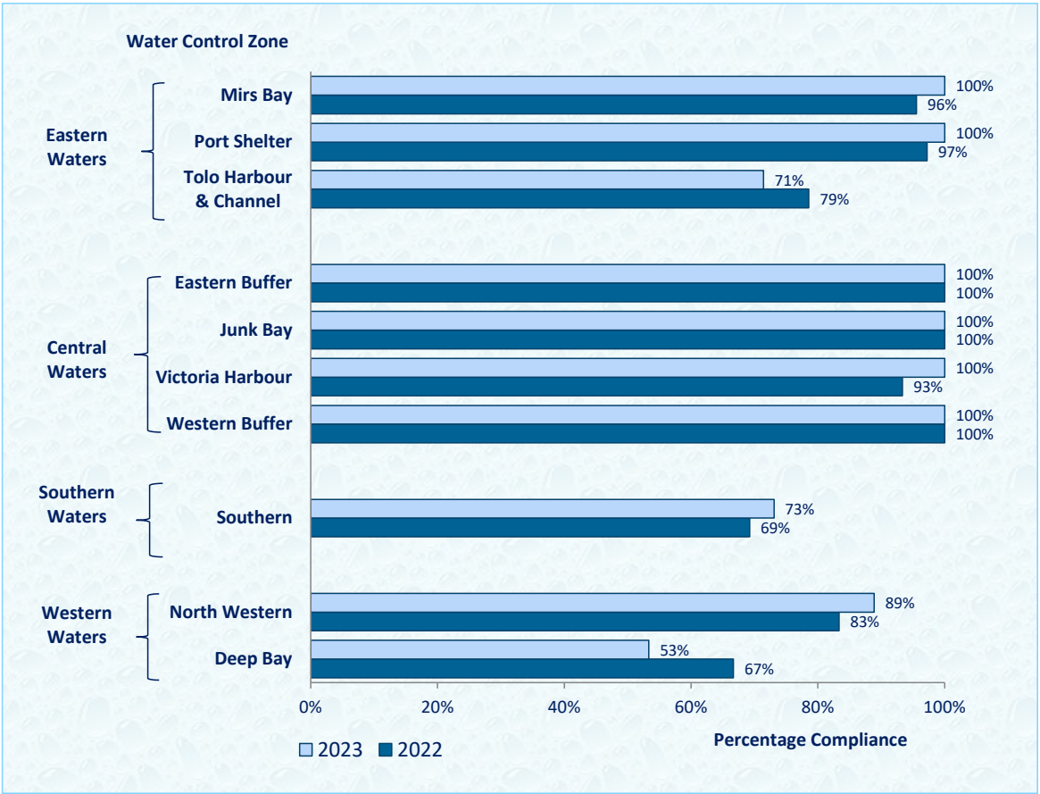
Figure 3. Marine WQO compliance rates for the ten WCZs, 2022-2023
