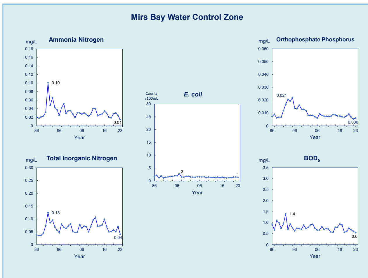
Figure 6. Long-term water quality trends in the Mirs Bay WCZ, 1986-2023
