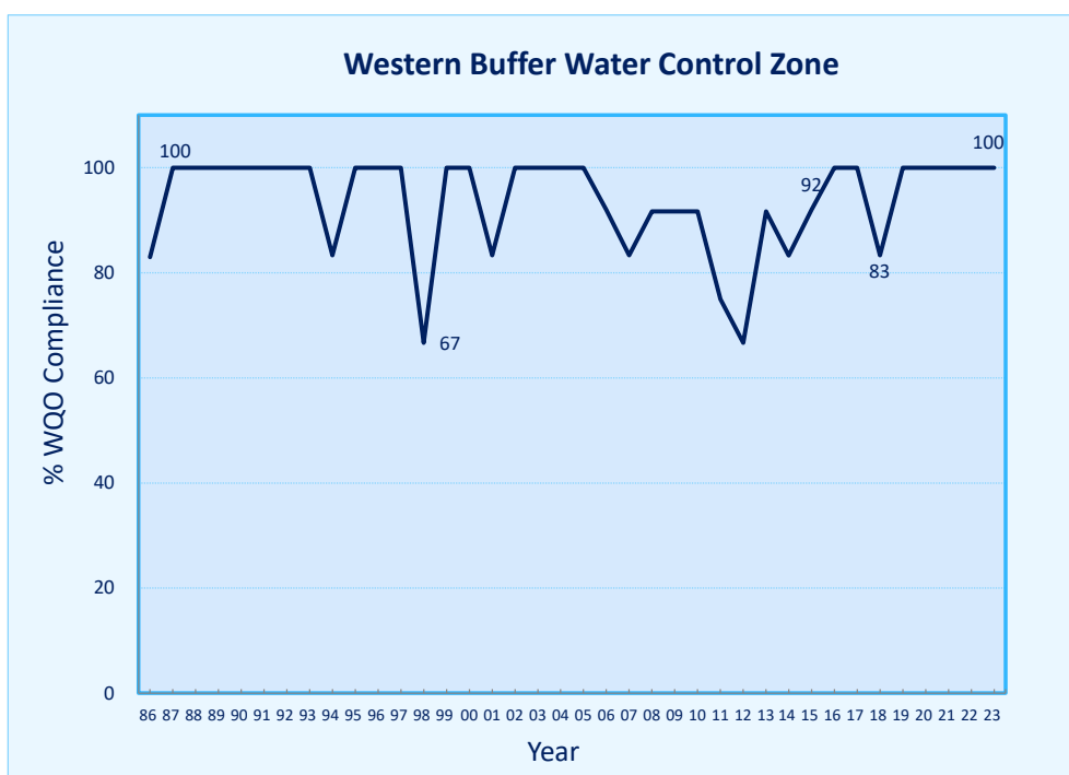
Figure 18. Overall WQO compliance rate for the Western Buffer WCZ, 1986-2023
