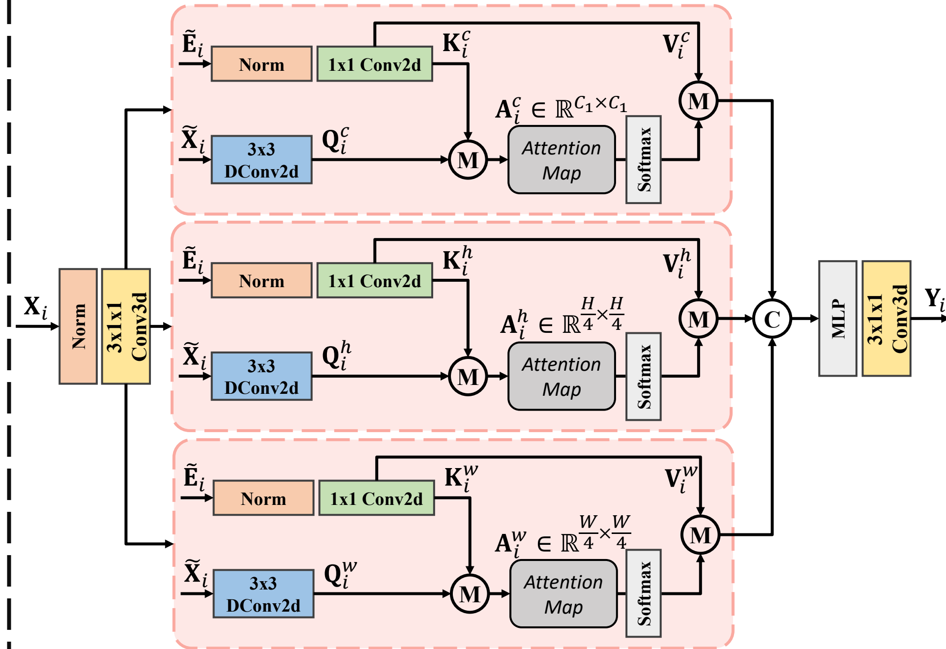
(b) Cross-Modal Collaborative Attention (CMCA)
