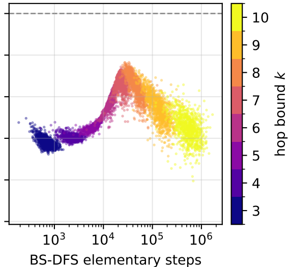
Watts-Strogatz
