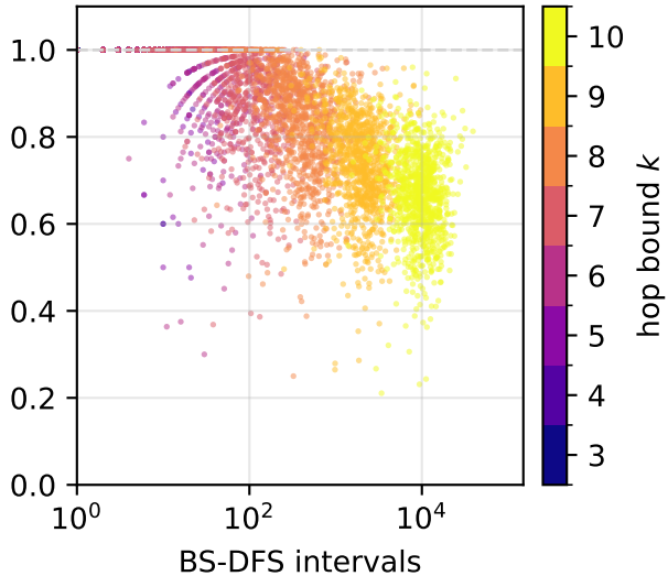
Watts-Strogatz
