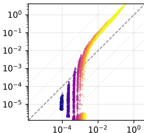
k-out
