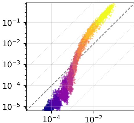
Watts-Strogatz
