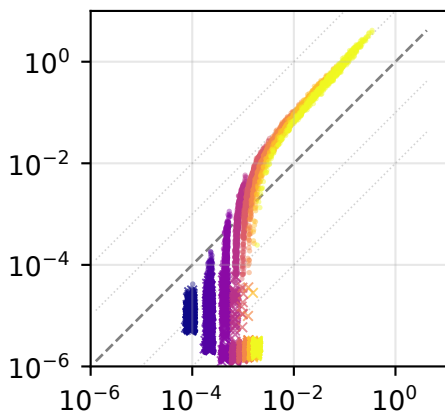
k-out
