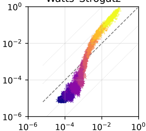
Watts-Strogatz
