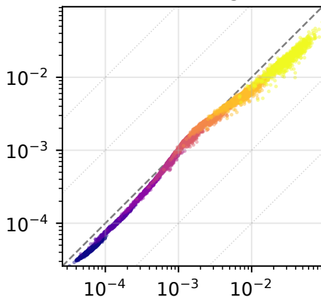
Watts-Strogatz
