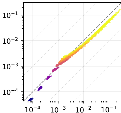
k-out
