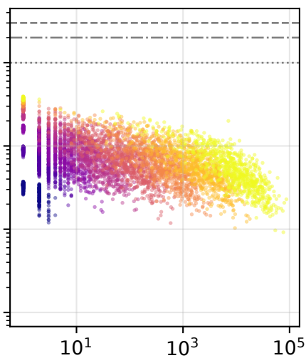
k-out
