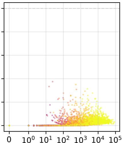
k-out
