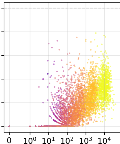
k-out
