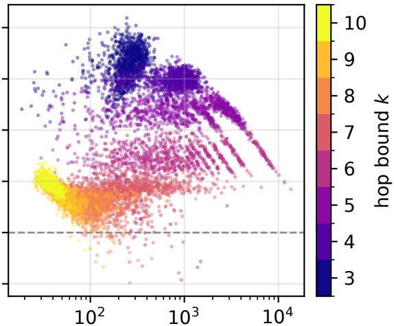
Watts-Strogatz
