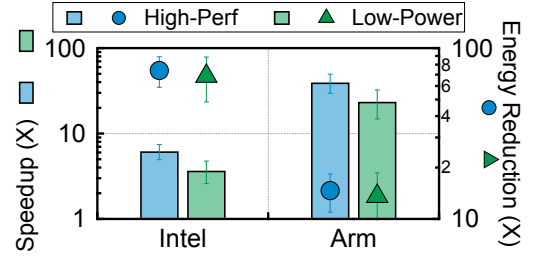
Fig. 16: Speedup and energy reduction of the two ARCHYTAS variants over the baselines. Error bars denote one stdev. No design in this figure uses the dynamic optimization.
