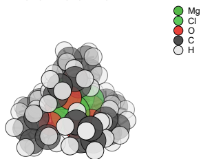
\text{Mg}^{2+} first shell [\text{Mg}_2(\mu\text{-Cl})_3(\text{THF})_6]^+
