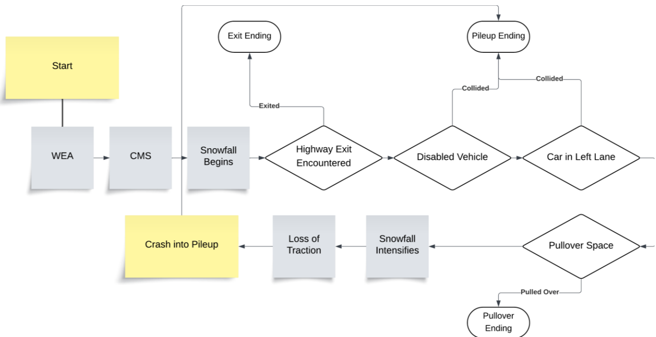
Fig. 1 General flow of the simulation.
