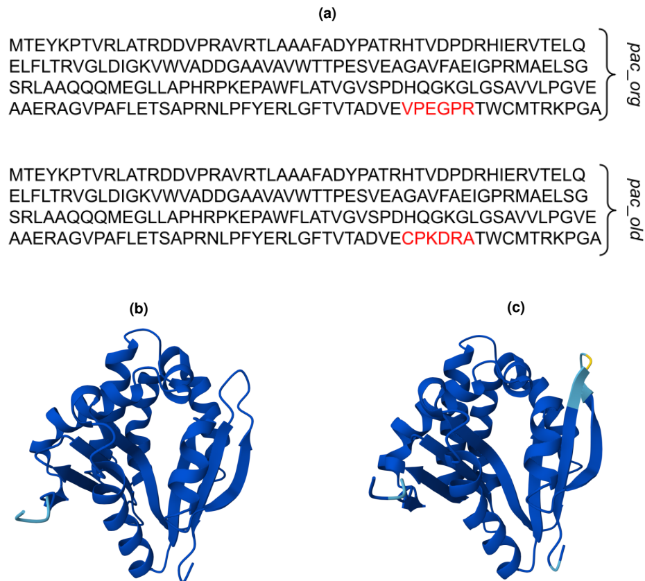
Figure 13: Aminoacids (AA) sequence of two pac genes and their 3-D structures. (a) shows the AA sequence of the original sequence from Streptomyces alboniger ( pac_org ) as well as from the pac gene that was located in the plasmid originally intended for transformation ( pac_old ). The differing section is highlighted in red. (b) The projected 3D structure for pac_org calculated by AlphaFold. (c) The projected 3D structure for pac_old calculated by AlphaFold. The color of the structure in AlphaFold shows the confidence of the predicted structure: blue, very confident, light blue less and yellow not very confident.
