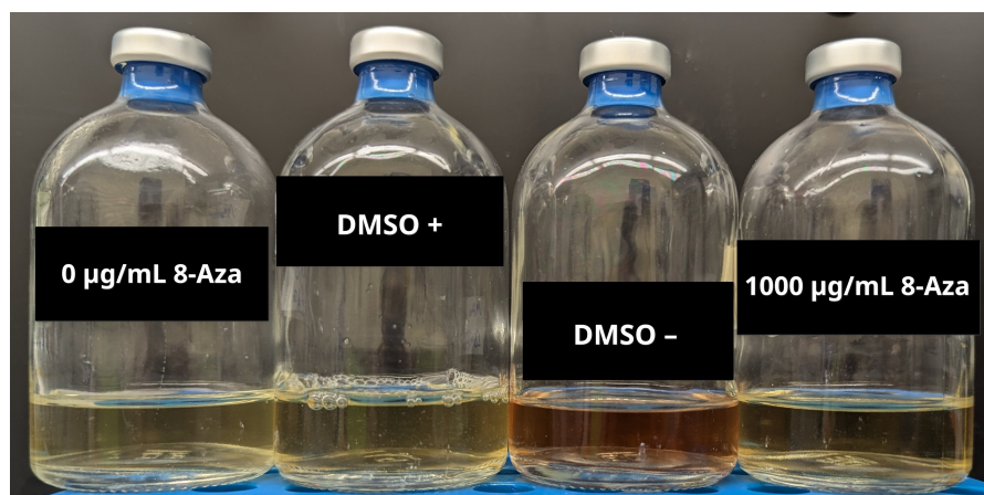
Figure 12: Color differences with and without DMSO after 6 days of incubation. Image of various preparations for M. thaueri from the same triplicate (Cltr. 3). The positive control (0 \mu\text{g/mL} 8-Azahypoxanthin (8-Aza)) contains only the microbe ( M. thaueri ) in DSM 1523; 1000 \mu\text{g/mL} preparation 8-Aza M. thaueri and the named base analog; DMSO + M. thaueri and 1 mL DMSO; DMSO – also contains 1 mL DMSO but was not inoculated.
