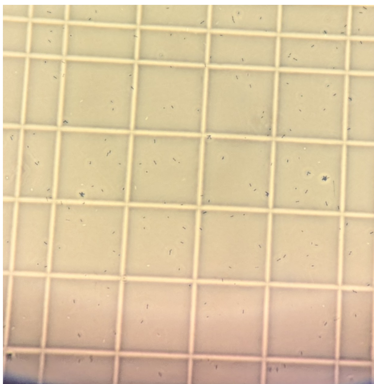
Figure A2: Phase-contrast microscope picture of Methanobrevibacter boviskoreani AbM4 at 400 times magnification. One group square with its sixteen small squares of a Neubauer improve counting-chamber is shown.
