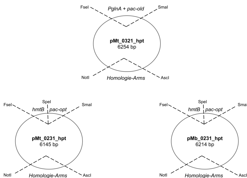
Figure 3: Suicide plasmid maps for transformation by conjugation for M. thaueri and M. boviskoreani . pMt_0321_hpt (6254 bp) is the parent plasmid used to construct the other two, pMt_0231_hpt (6145 bp) and pMb_0231_hpt (6214 bp). The maps show only the gene regions (between the dashed lines) that have been modified, as well as the restriction site sites (at the end of the dashed lines) used or the newly created restriction site sites. The new produced plasmids were verified via nanopore sequencing.
